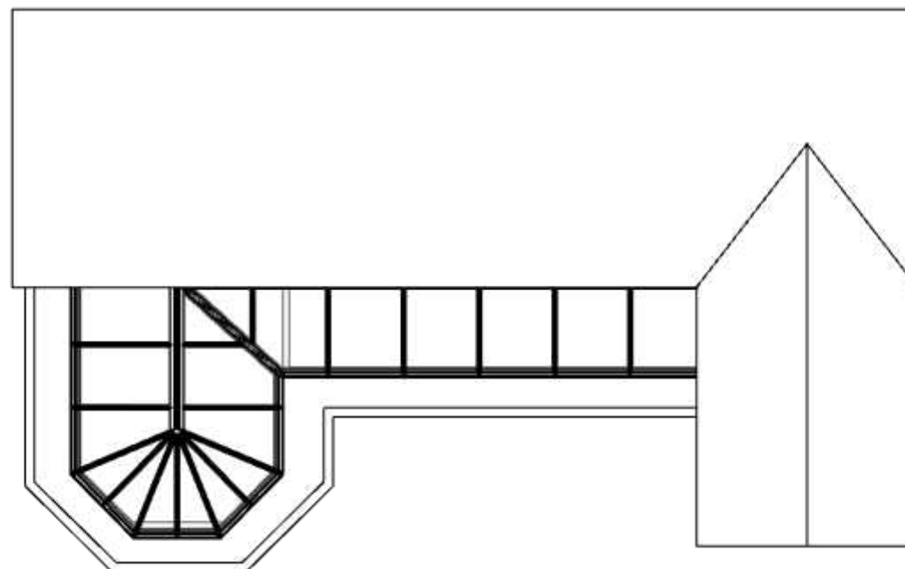
Proposed Roof Plan (Part)
