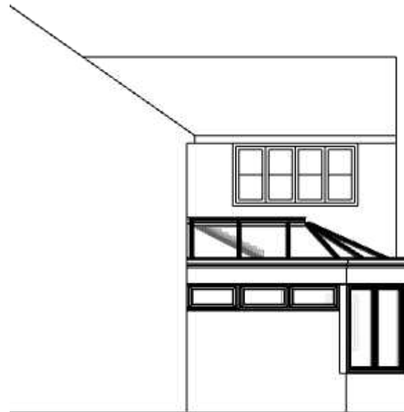
Proposed Left Side Elevation (Part)
