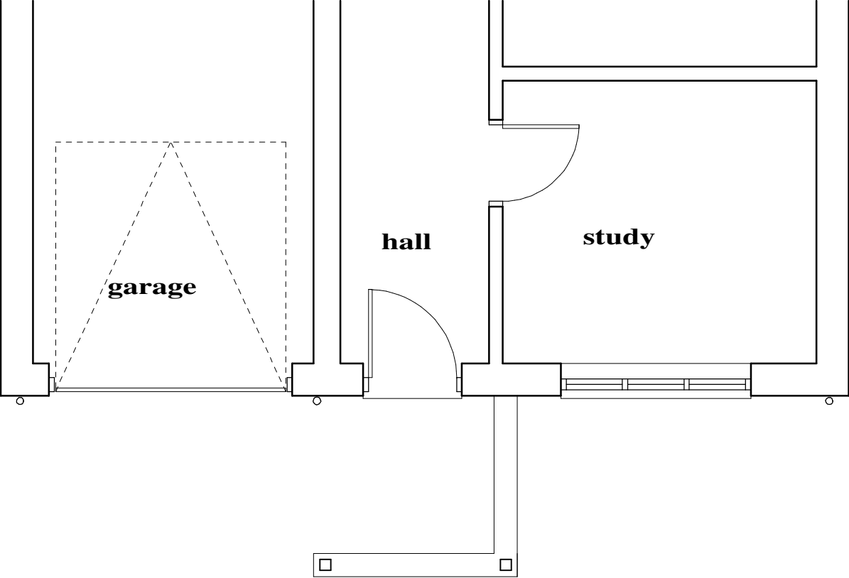
Existing Part Ground Floor Plan
