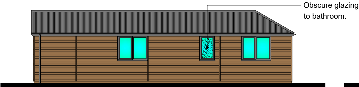
North east elevation. Scale 1:100
