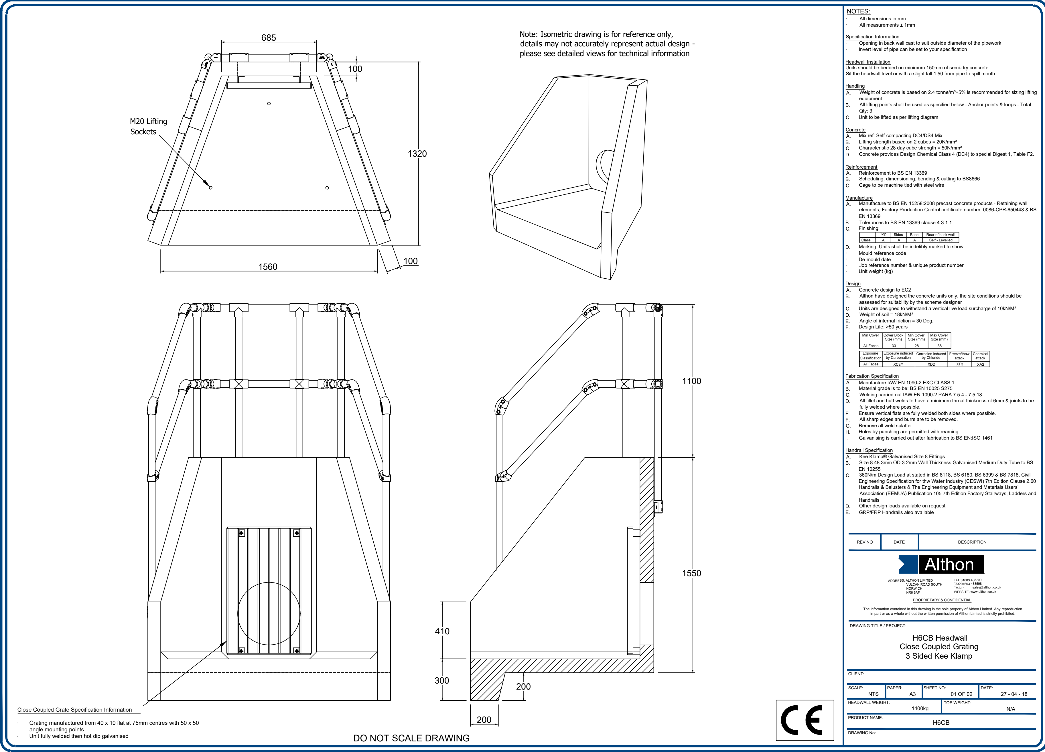
Headwall Detail - HW9, HW10 1:20 BASED ON ALTHON SFA 27B (OR SIMILAR APPROVED)
