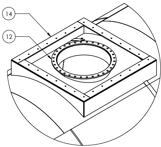
SQUARE UPSTAND DETAIL A SCALE 1 : 25
