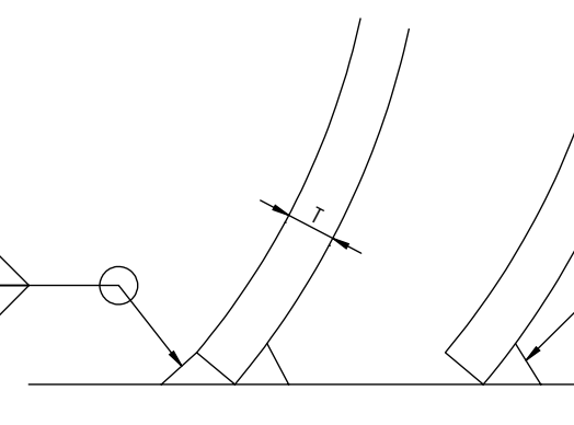
TWIN COMPARTMENT HEAD WELD DETAIL
