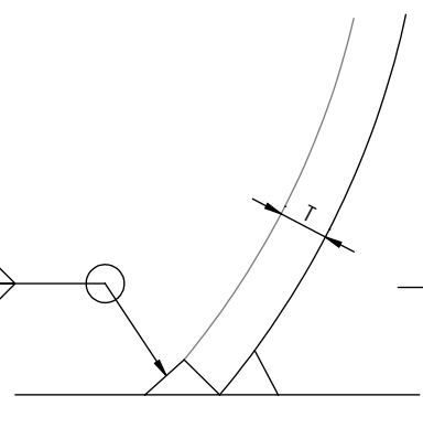
COMPARTMENT HEAD WELD DETAIL FOR INTERNALLY LINED TANKS
