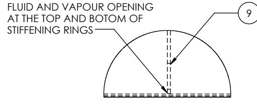
STIFFENING RING DETAIL G SCALE 2 : 25
