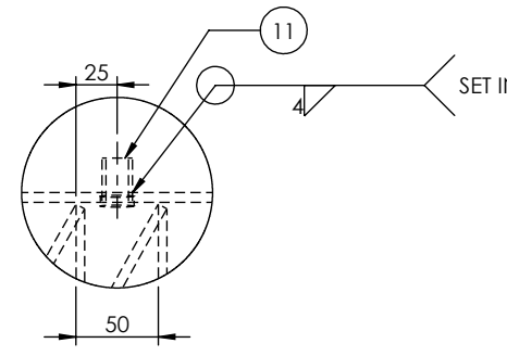
LEAK DETECTION TWIN COMP HEADS DETAIL I SCALE 1 : 5
