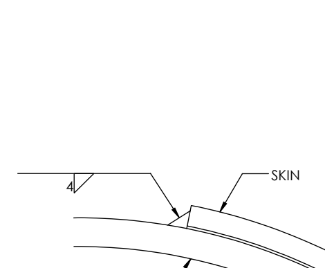
SKIN PLATE WELD DETAIL
