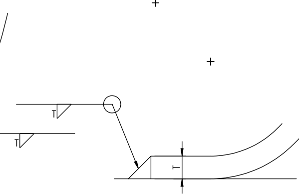
SINGLE COMPARTMENT HEAD WELD DETAIL
