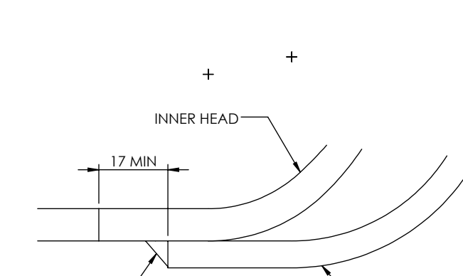
SKIN DISHED HEAD WELD DETAIL
