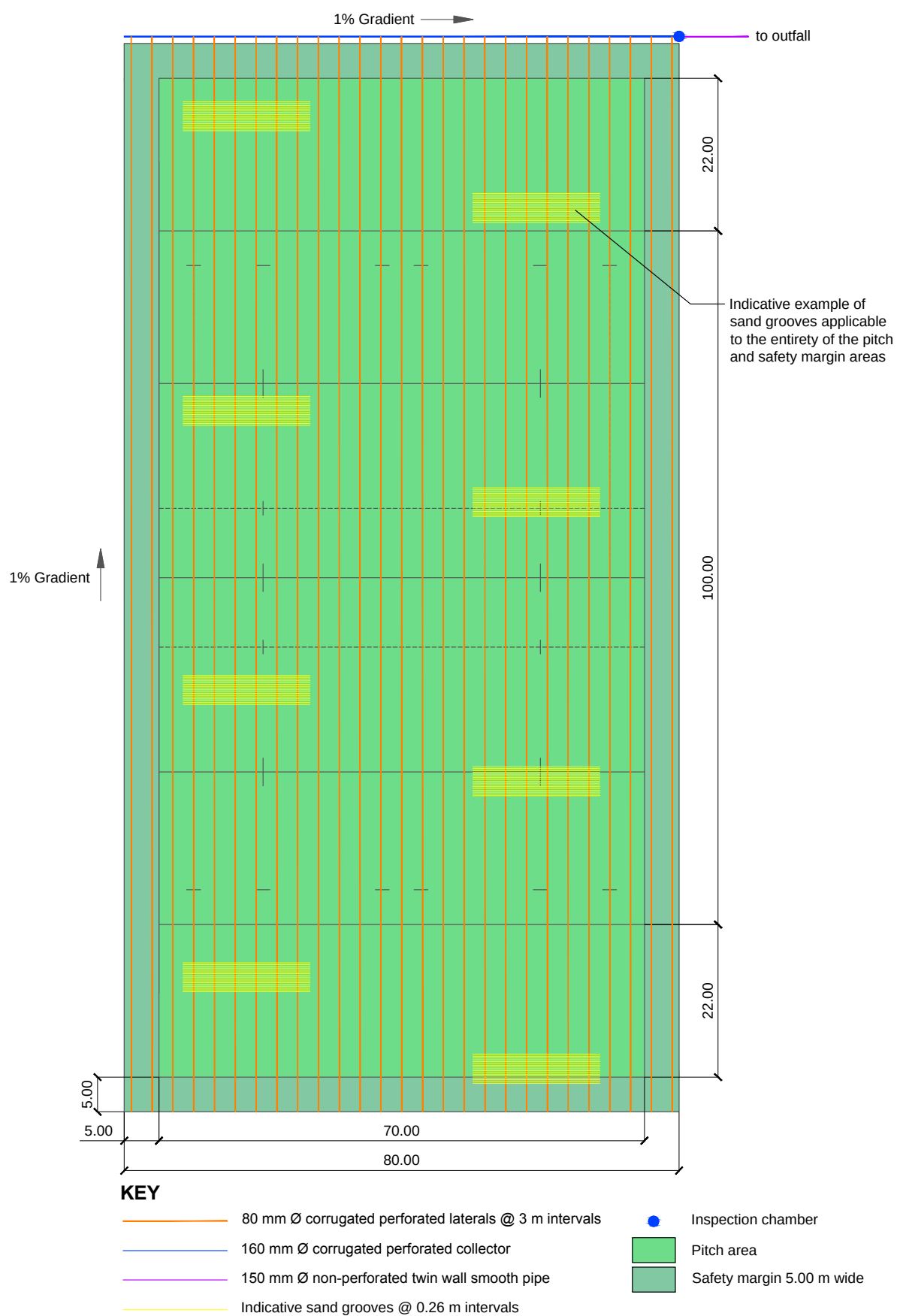
Playing area for Senior Rugby Union (100.00 m x 70.00 m) - standard layout with sand grooves
