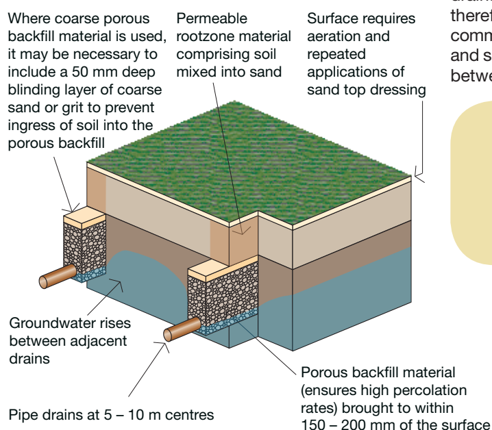
Pipe drainage construction on cultivated topsoil
