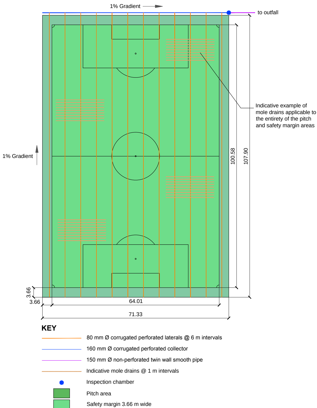
Playing area for Senior football (100.58 x 64.01 m) - standard layout with mole drains
