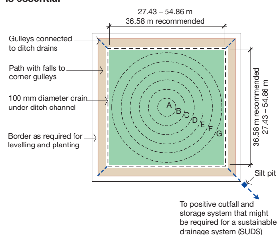
Crown green showing contours and ditch drain
