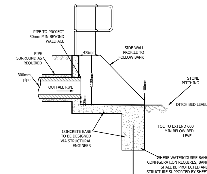
SECTION - A
