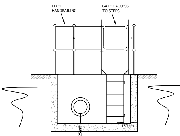
SECTION - B
