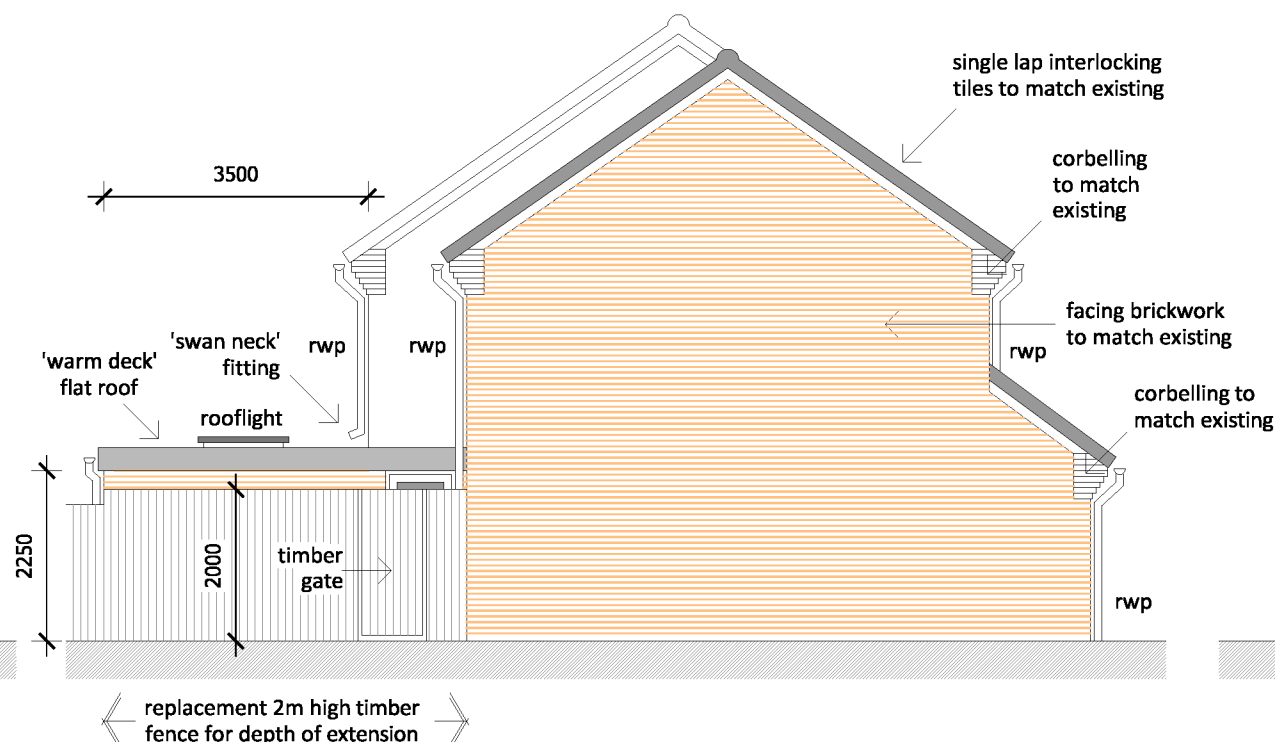
PROPOSED Side Elevation - East Facing
