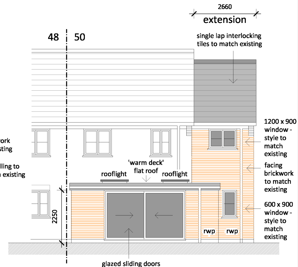
PROPOSED Rear Elevation - South Facing
