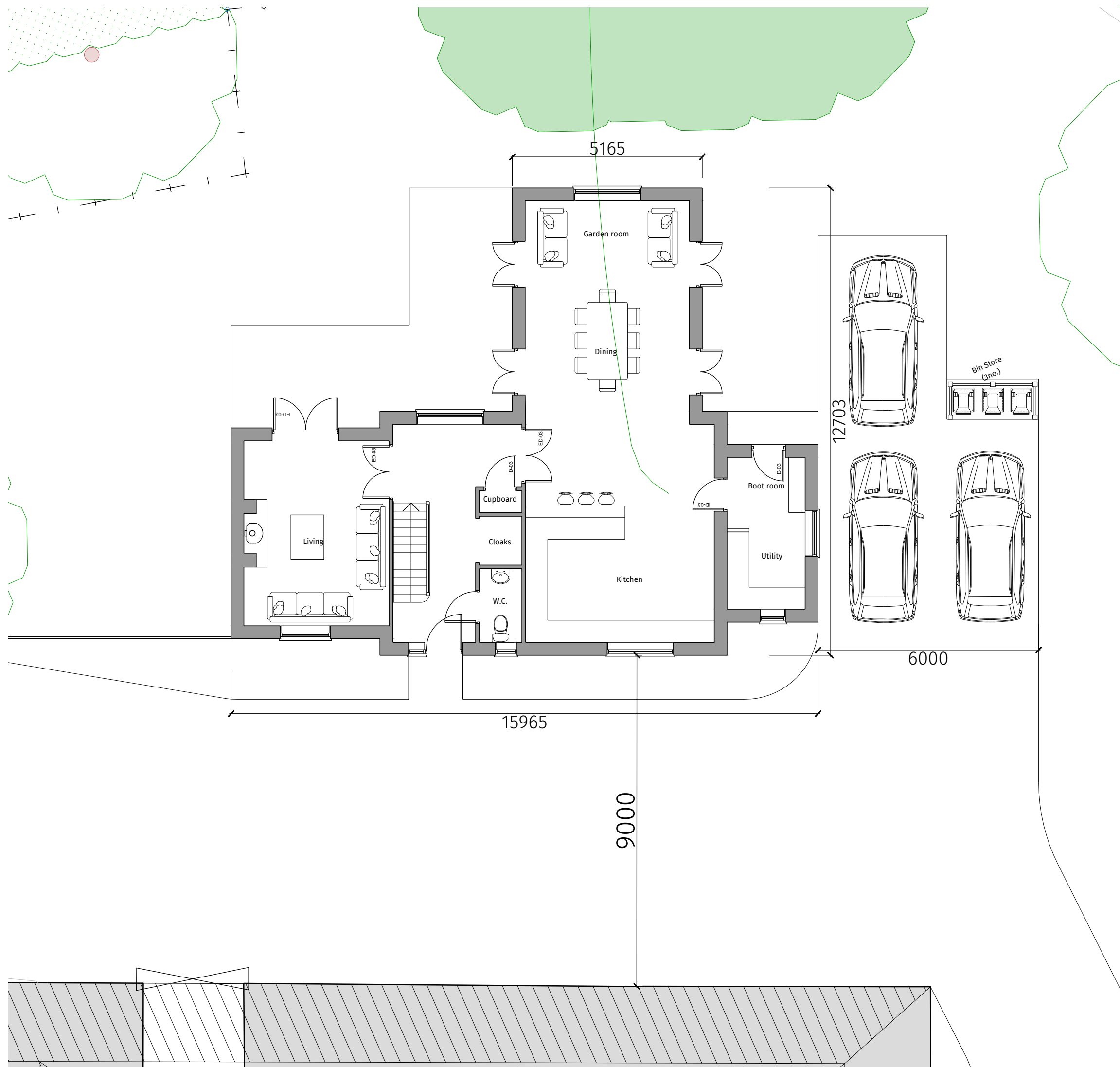
Ground Floor Plan (in context)
