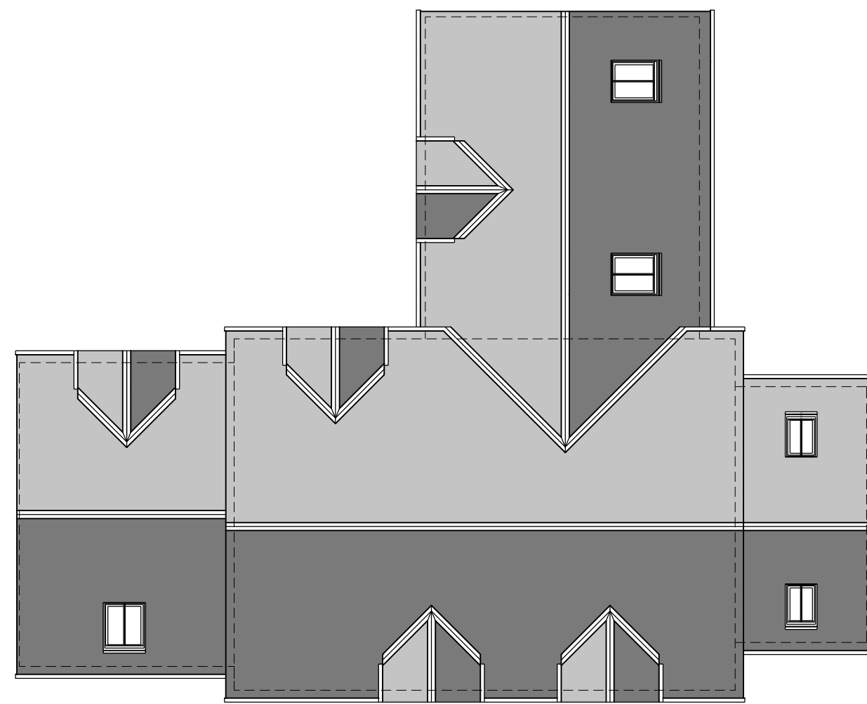
Roof Plan
