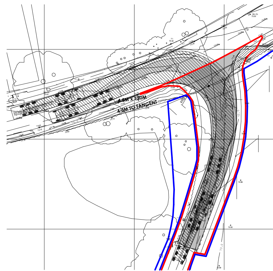
Access Block Plan - 1:500
