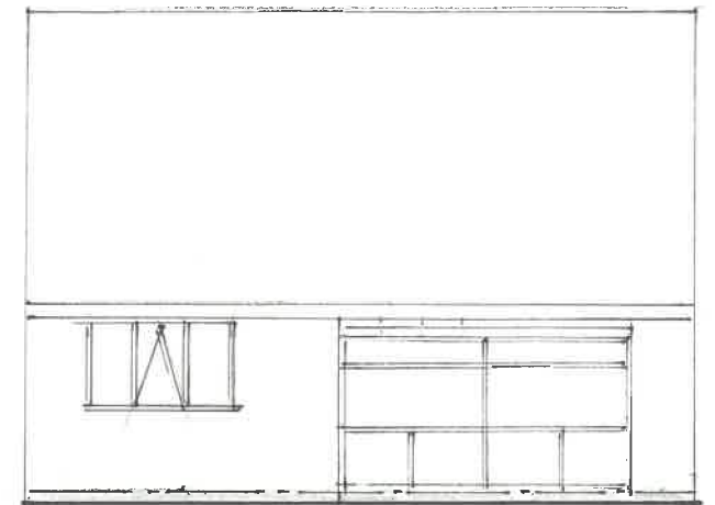
N/E FACING REAR ELEVATION
