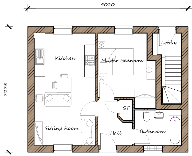
AF12GA-5 Ground Floor Plan
