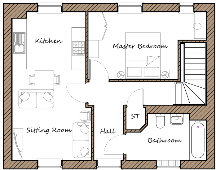
AF12GB-5 First Floor Plan
