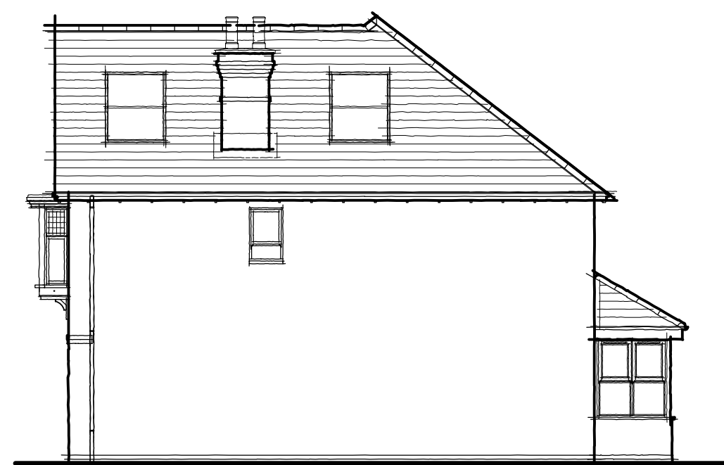
Side Elevation
