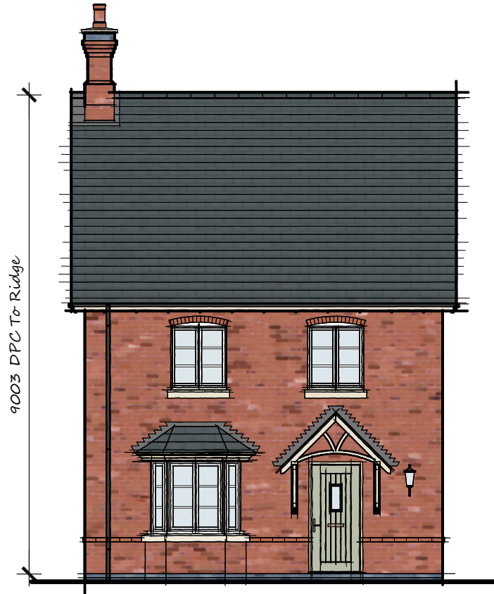
Front Elevation
