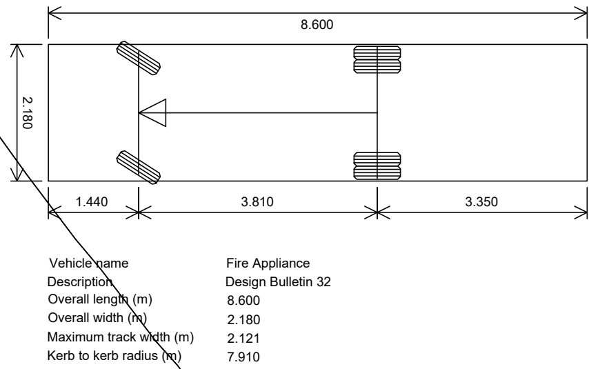
FIRE APPLIANCE TRACKING VEHICLE
