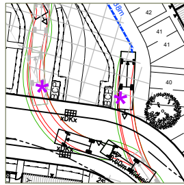
DENOTES FIRE TRACKING
