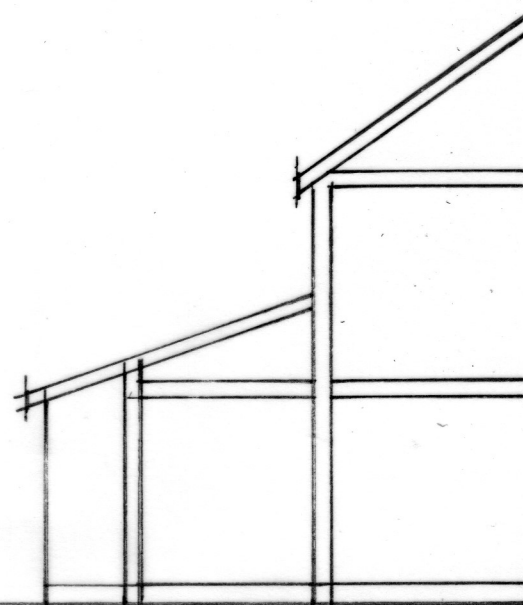
SIDE ELEVATION/SECTION
