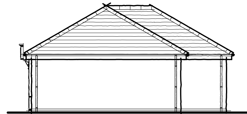
Side Elevation
