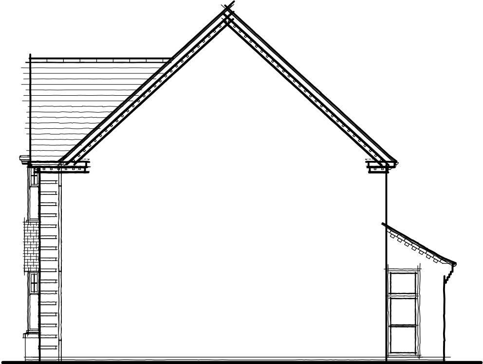
Side Elevation
