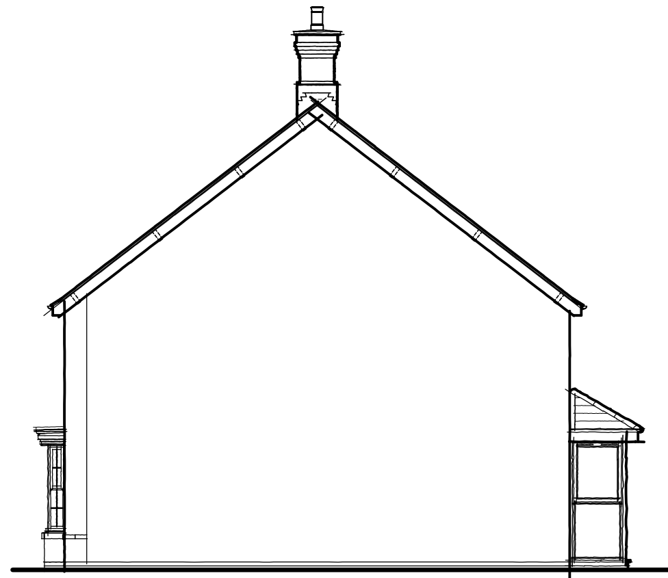
Side Elevation
