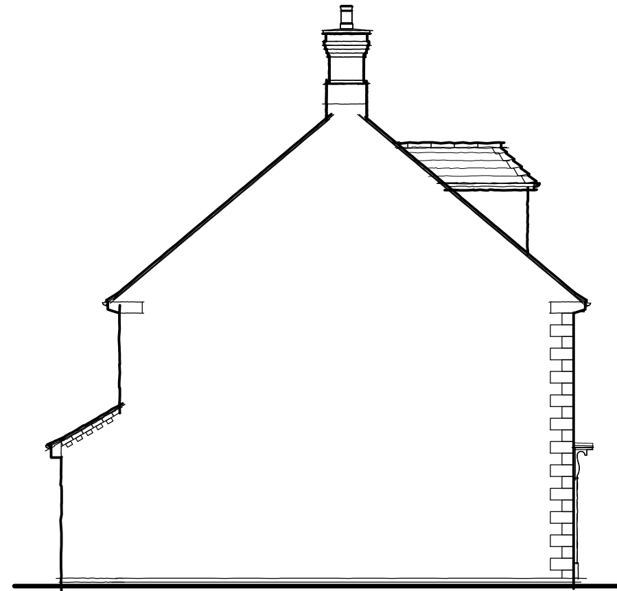
Side Elevation
