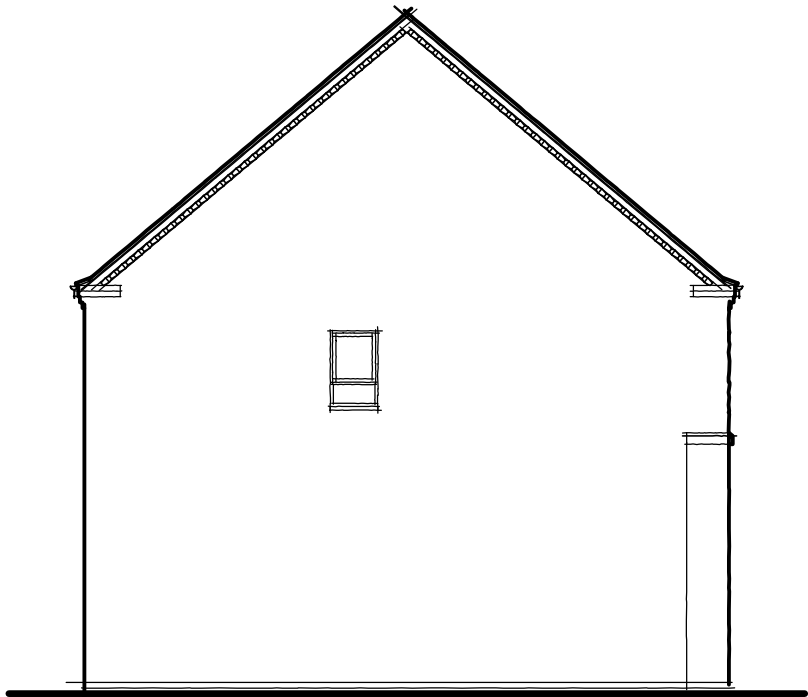
Side Elevation
