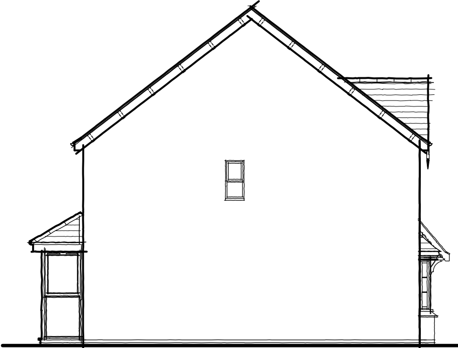
Rear Elevation
