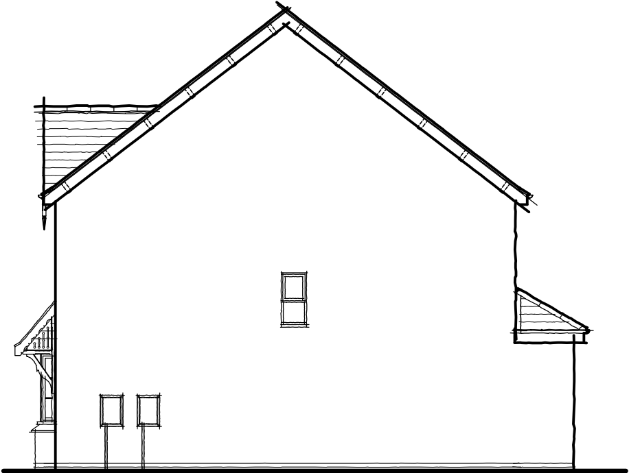
Side Elevation
