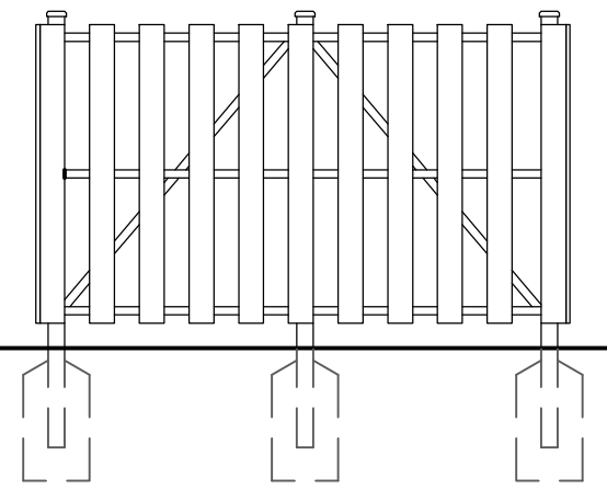
Bin store - rear elevation
