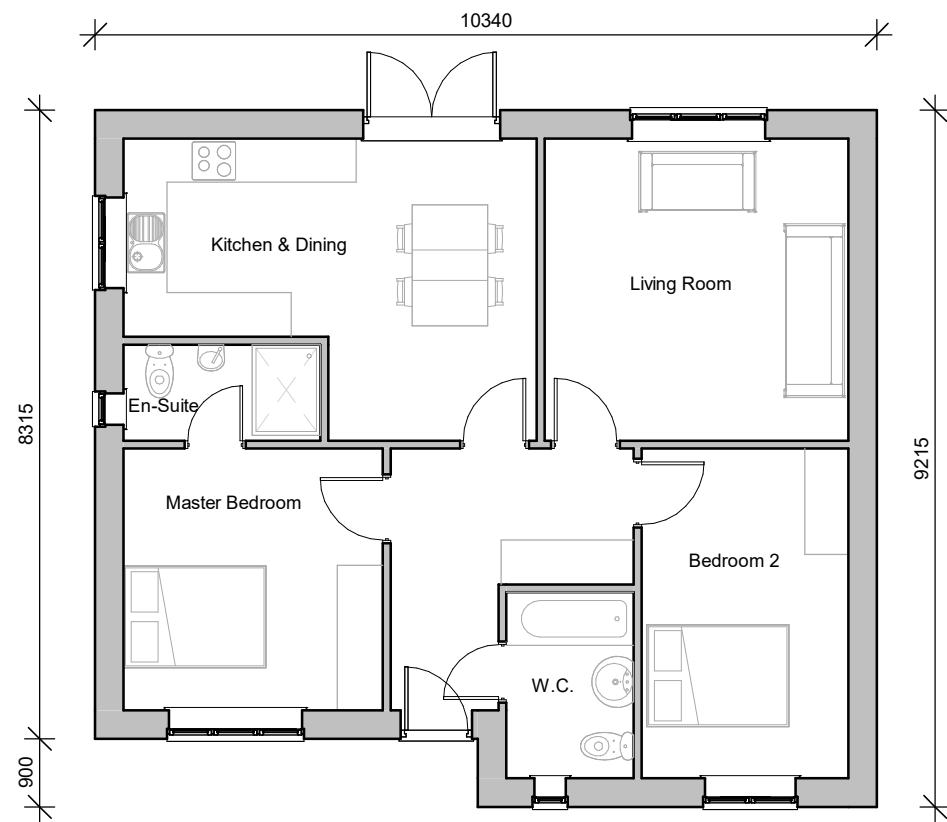
Ground Floor
