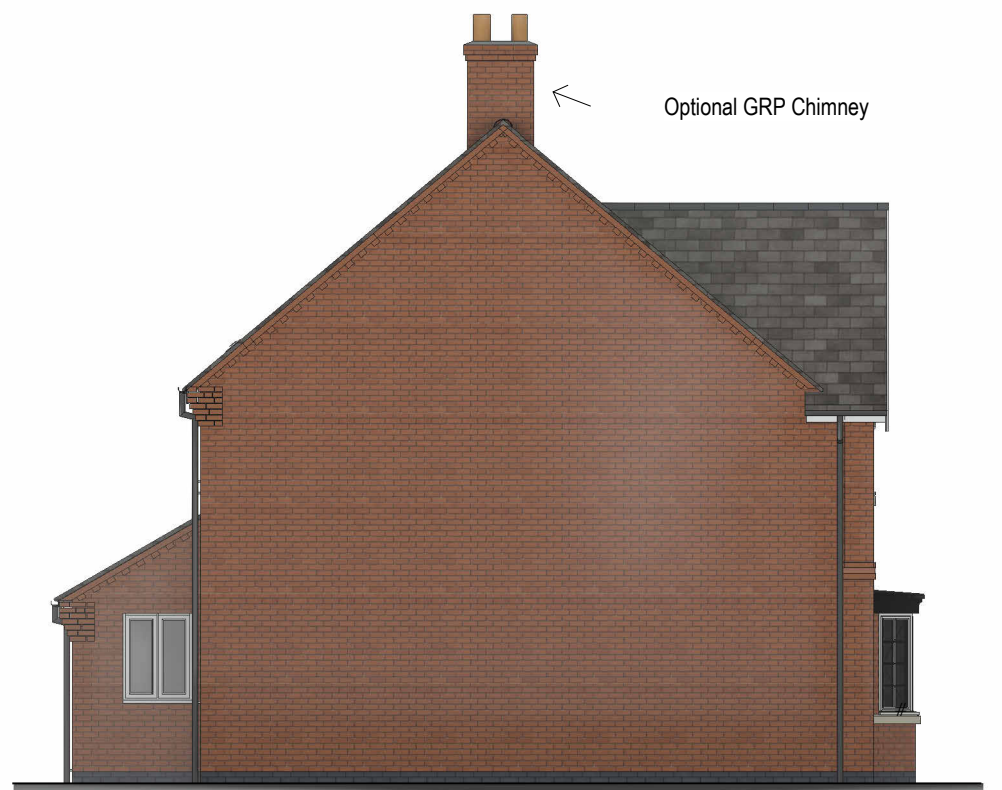
Side 1 Elevation
