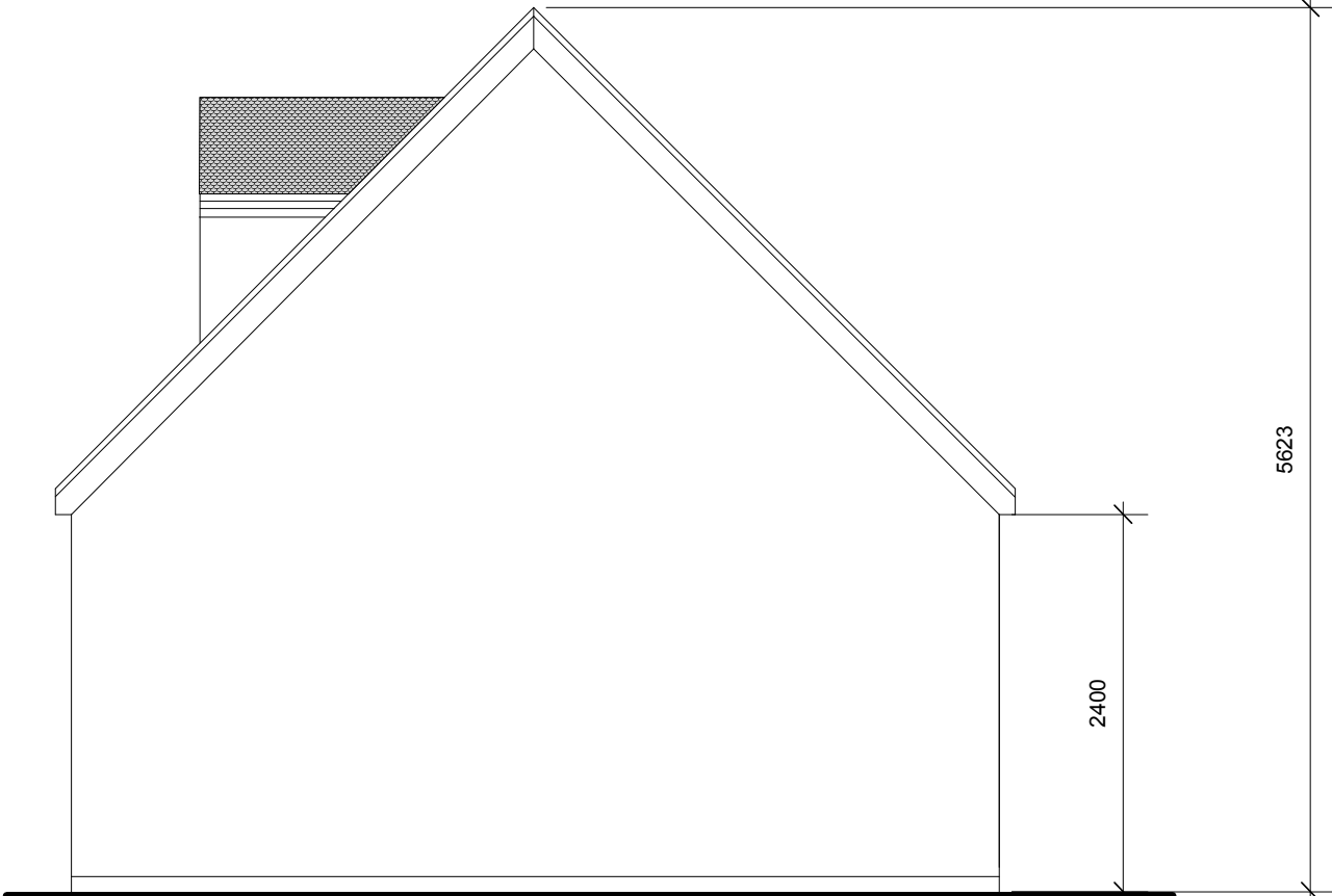
SIDE ELEVATION
