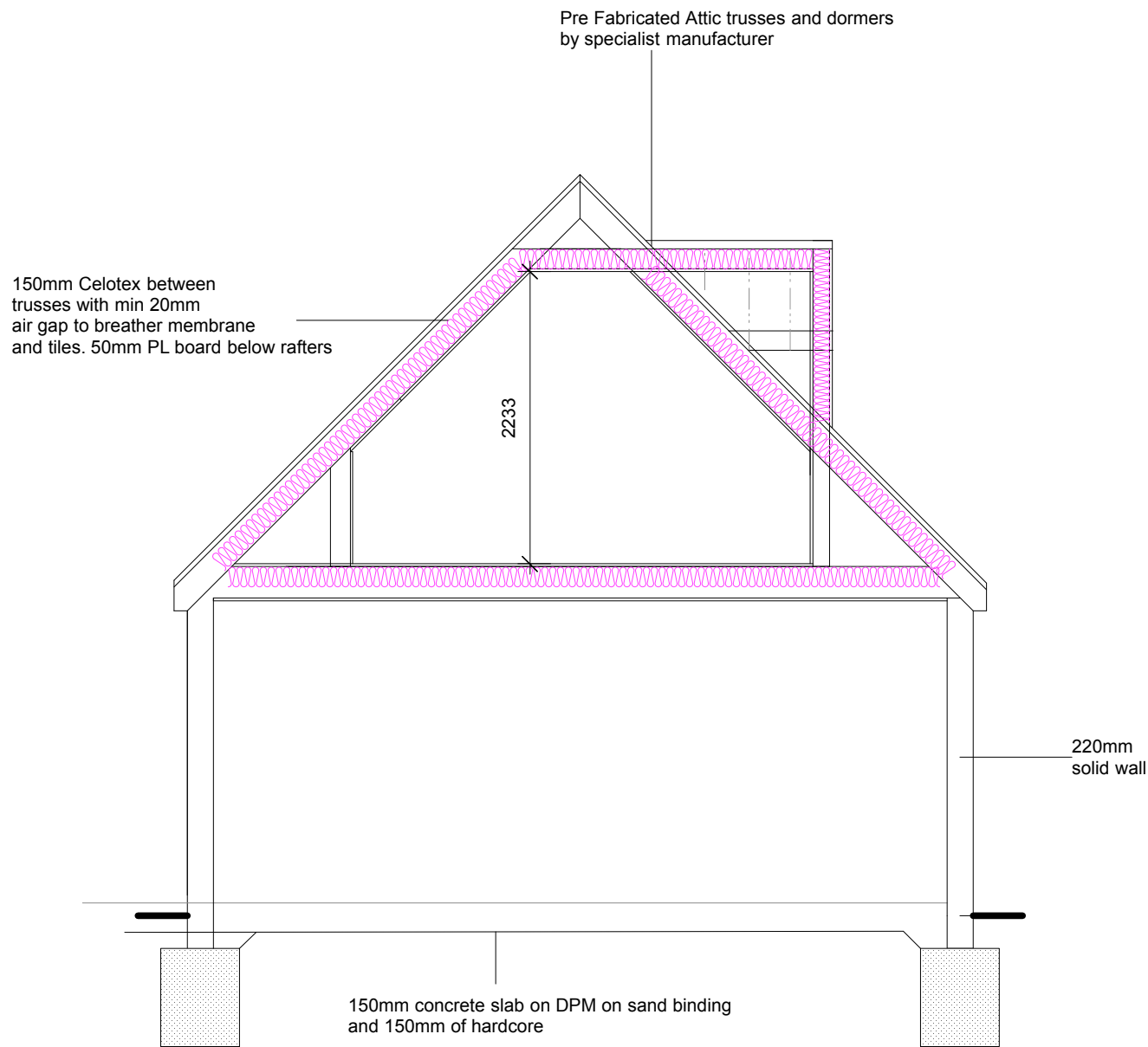
SECTION:
