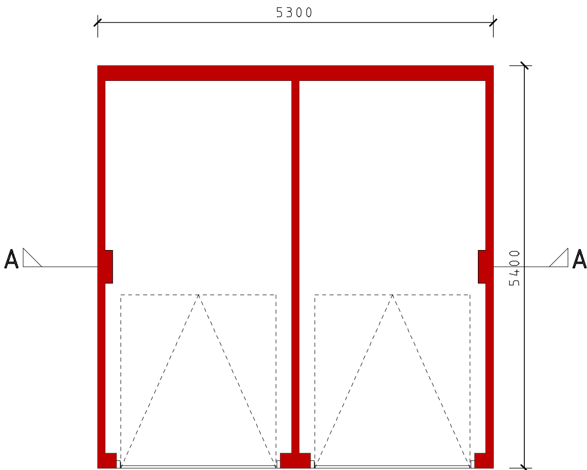
Floor Plan
