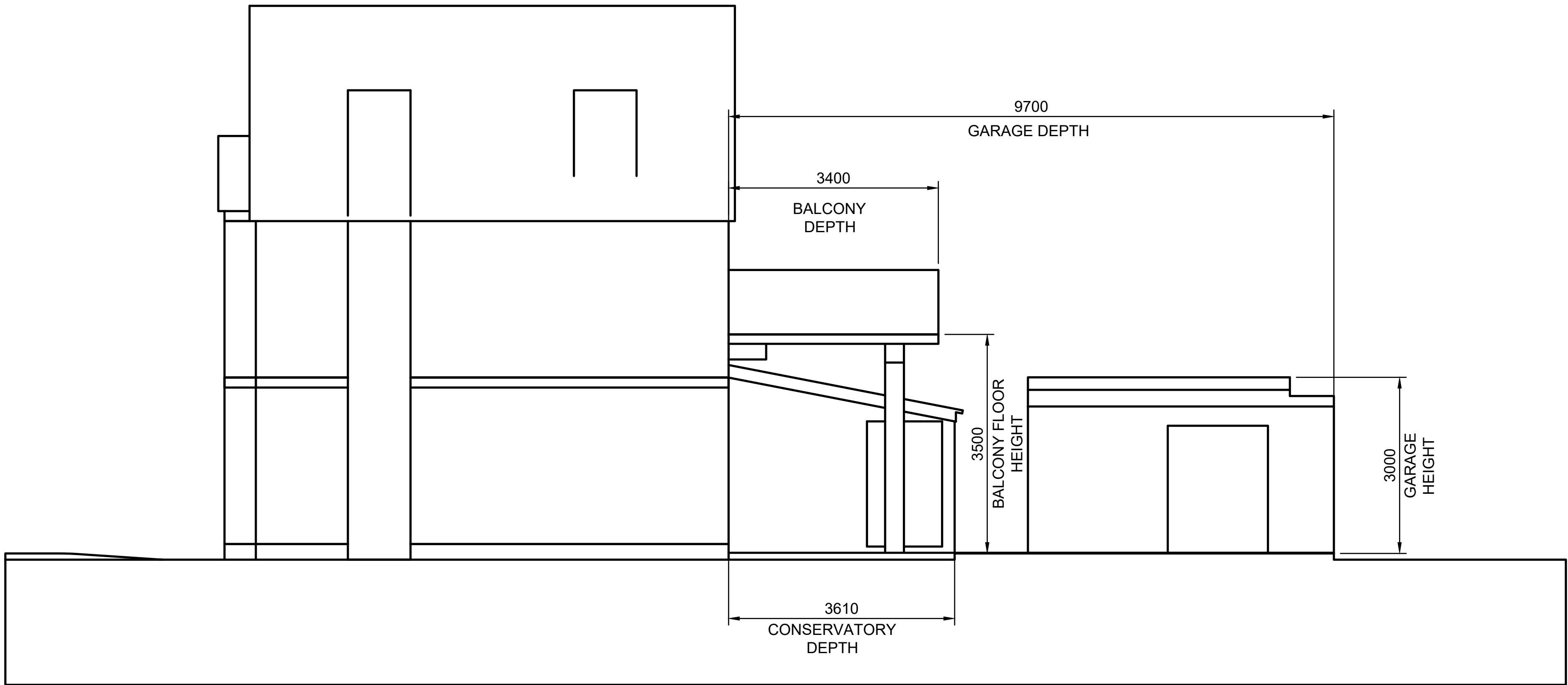
EXISTING SIDE ELEVATION SCALE 1:50
