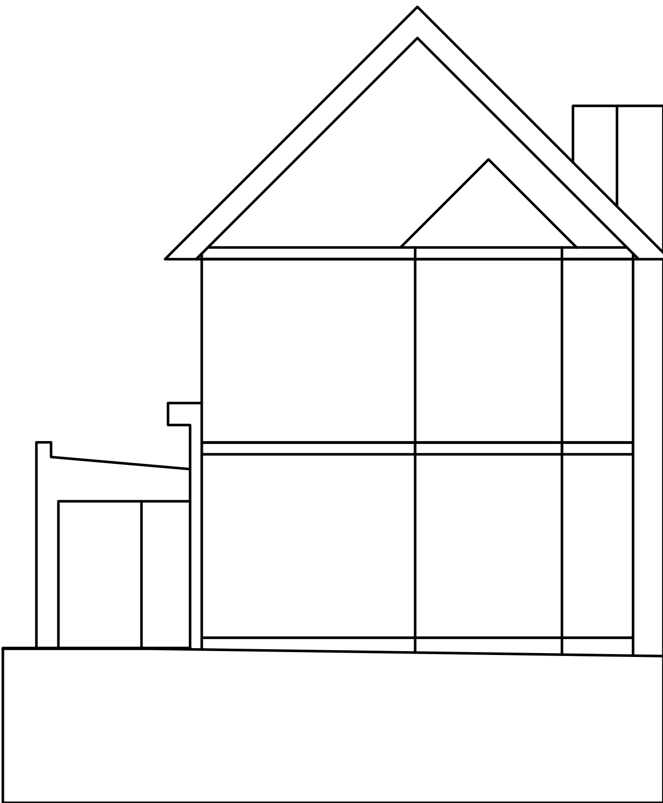
EXISTING FRONT ELEVATION SCALE 1:50
