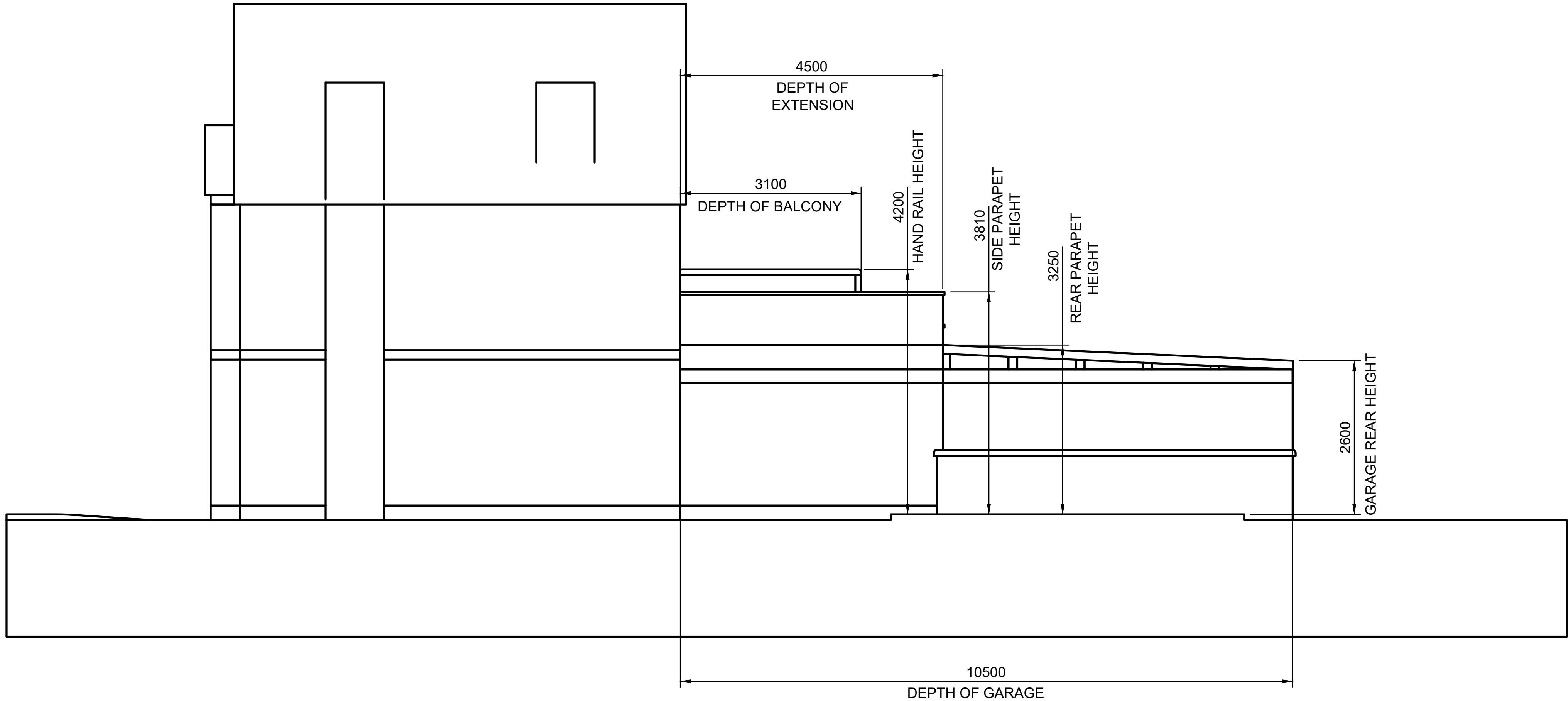
PROPOSED SIDE ELEVATION SCALE 1:50
