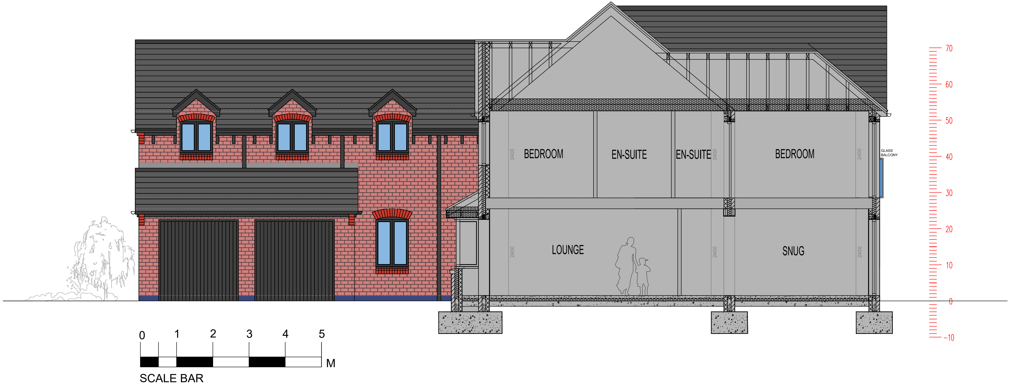
Existing Detailed Section A-A SCALE 1:50 @ A1
