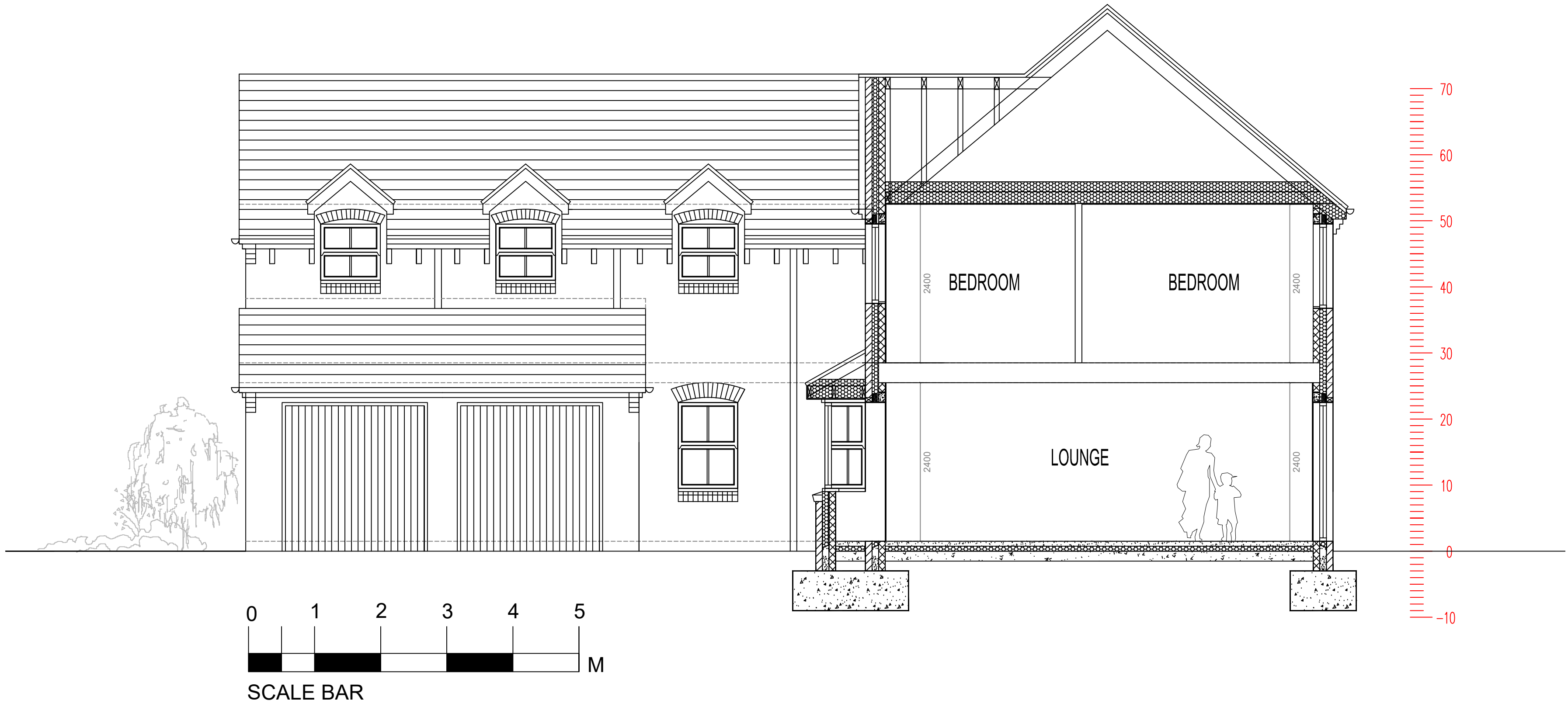
Existing Detailed Section A-A SCALE 1:50 @ A1
