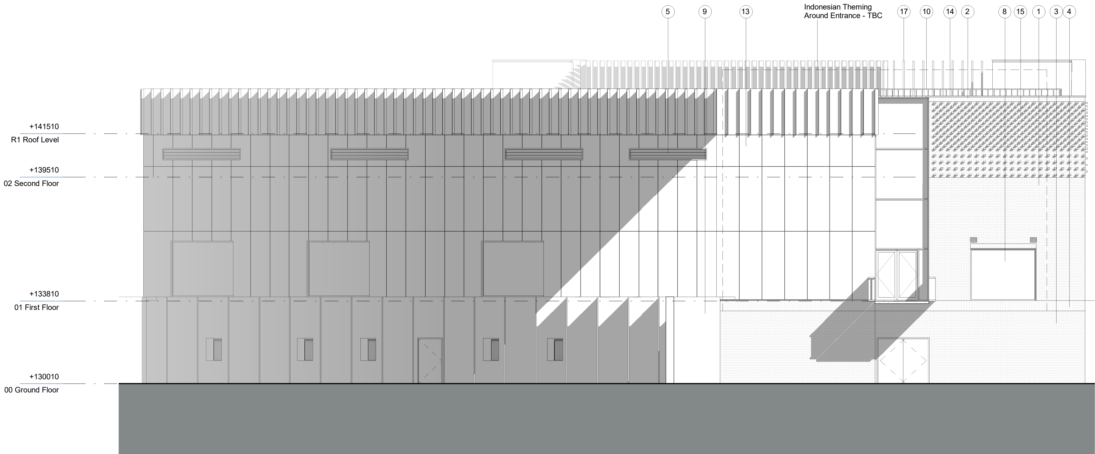
Elevation C: East Scale: 1 : 100
