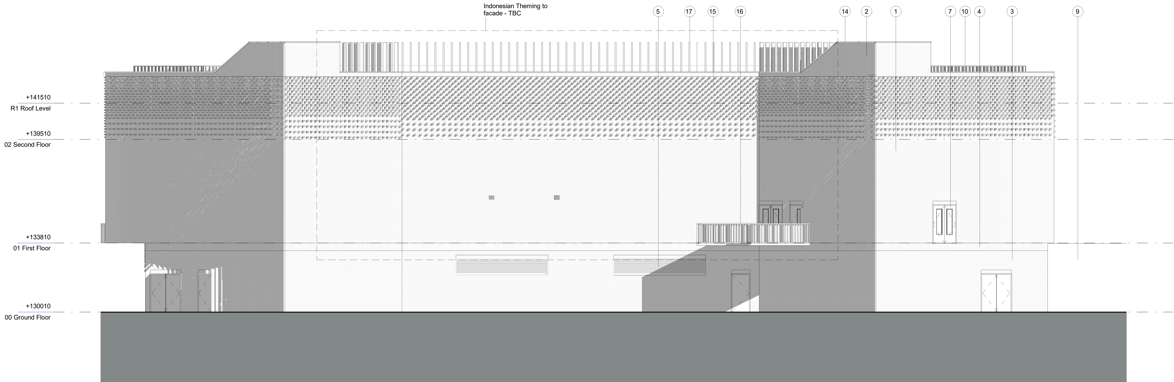
Elevation D: North West Scale: 1 : 100
