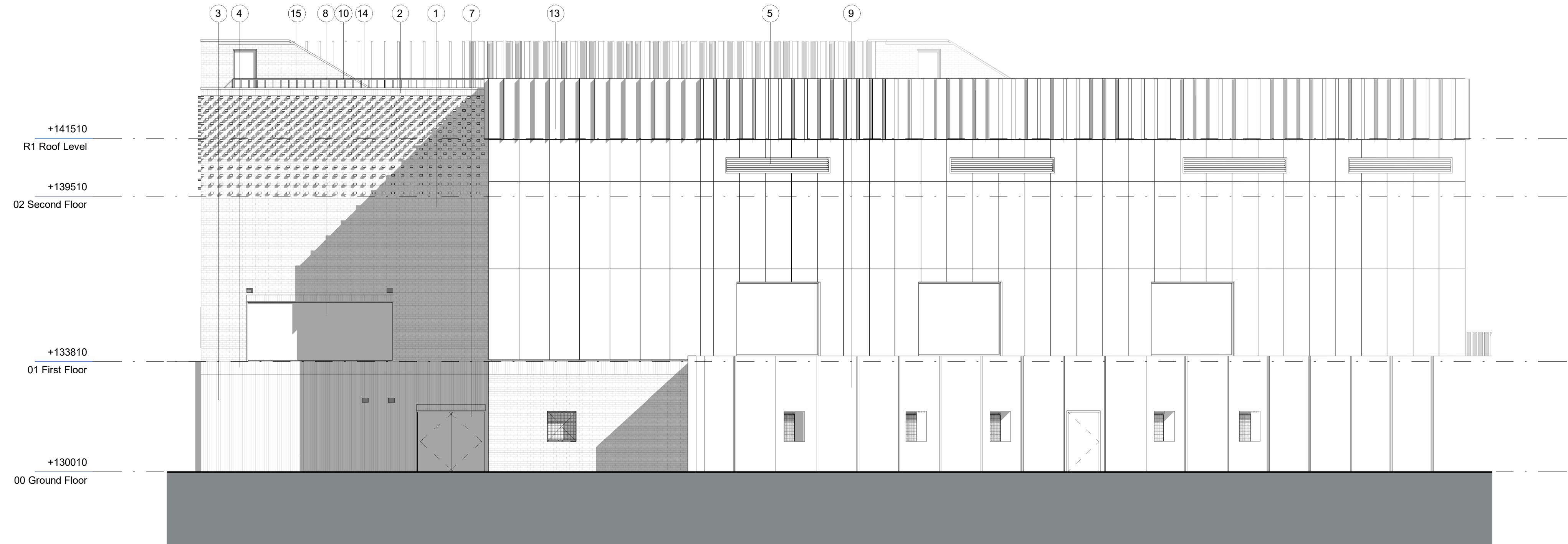
Elevation B: South Scale: 1 : 100
