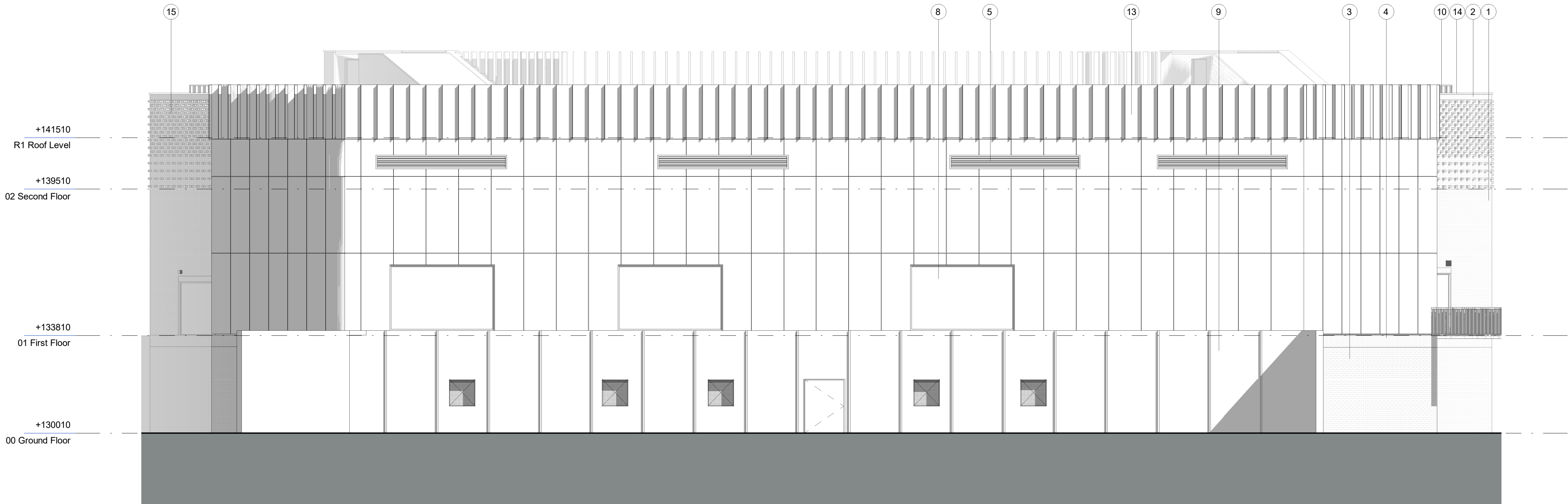
Elevation A: South East Scale: 1 : 100
