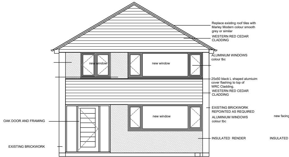
FRONT ELEVATION
