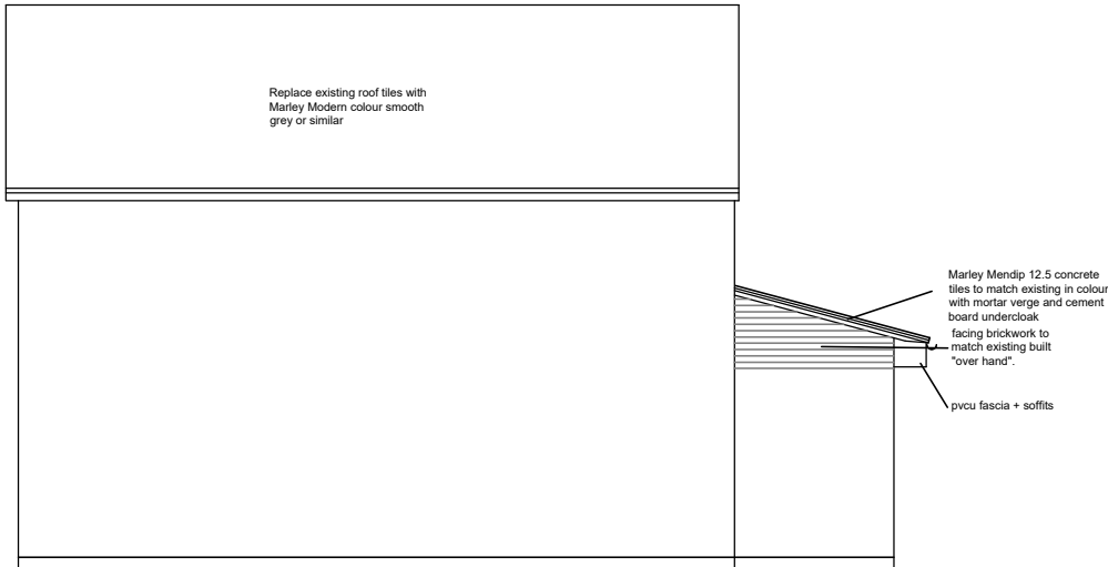
EAST SIDE ELEVATION
