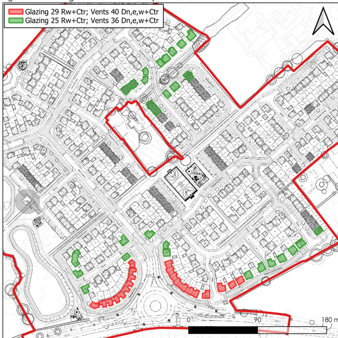
Figure 5.1: Glazing and Ventilation Requirements
