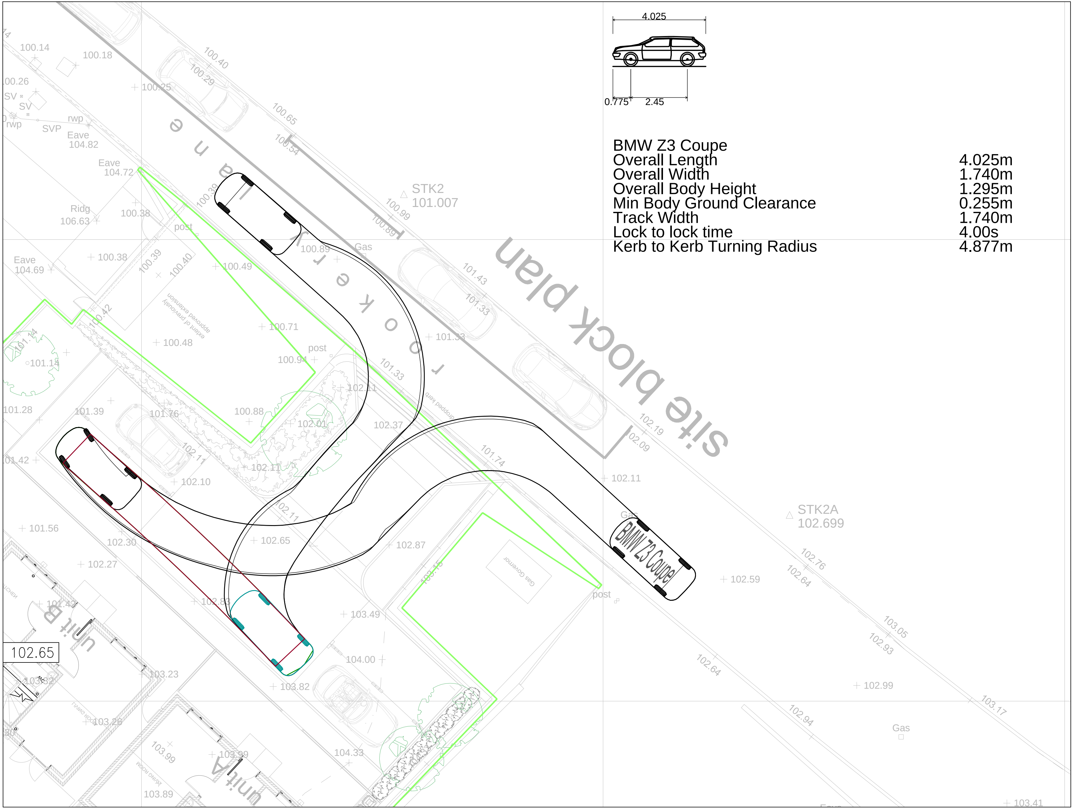
S184 Swept Path Scale 1:100
