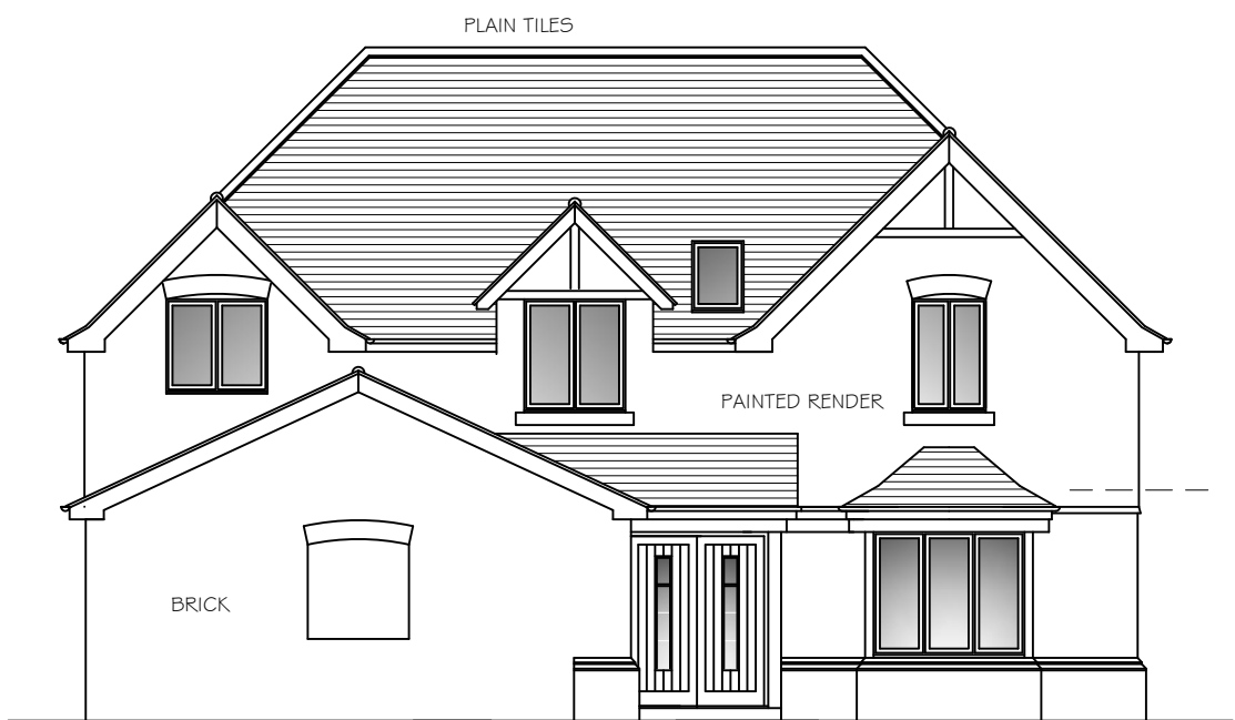
FRONT
