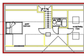
First Floor Plan Plot Five
