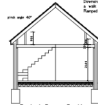
Typical Cross Section Scale 1:50
