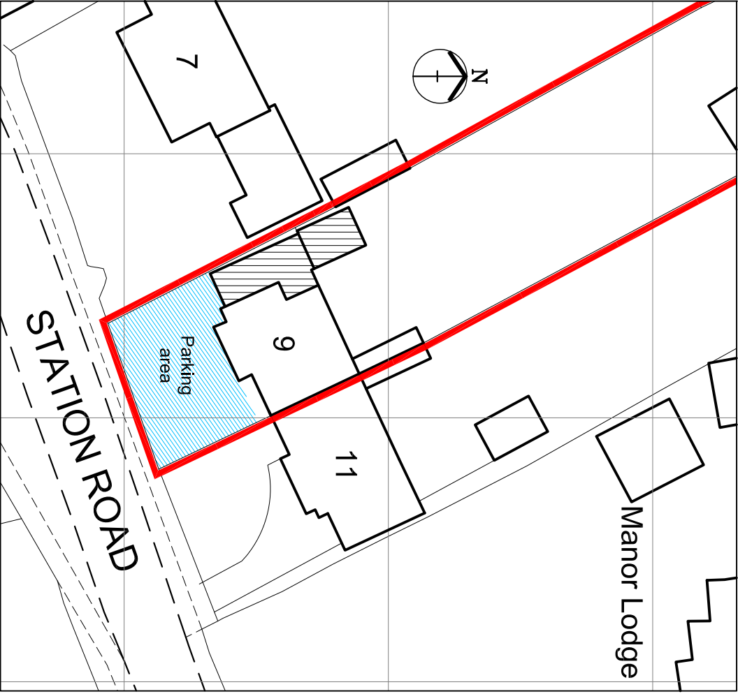
PROPOSED PARKING PLAN
