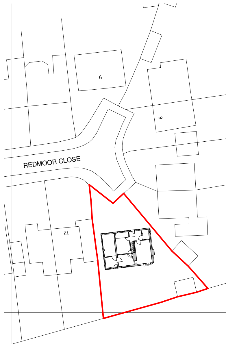
As Existing Block Plan Scale @ 1:500
