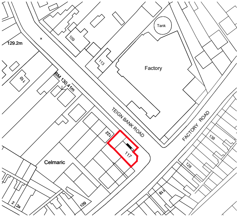
Proposed Site Location Plan 1:1250
