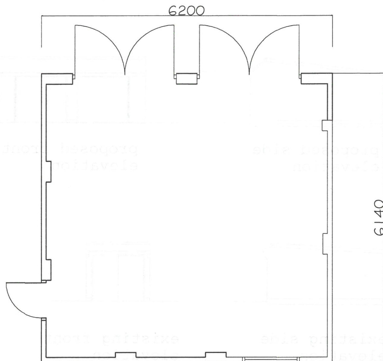
proposed plan
