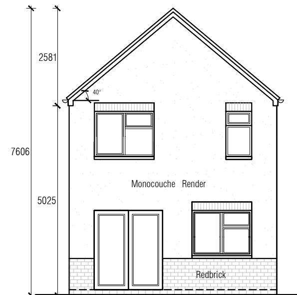
PROPOSED REAR ELEVATION.PLOT 2
