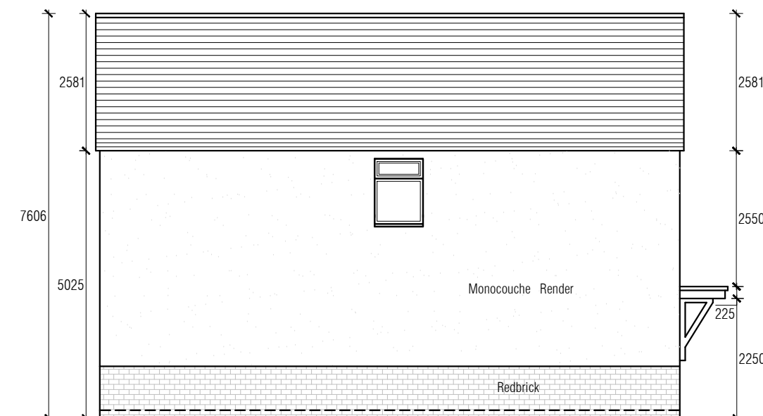
PROPOSED SIDE ELEVATION LHS .PLOT 2
