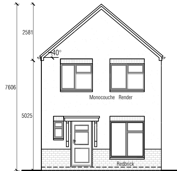
PROPOSED FRONT ELEVATION.PLOT 2
