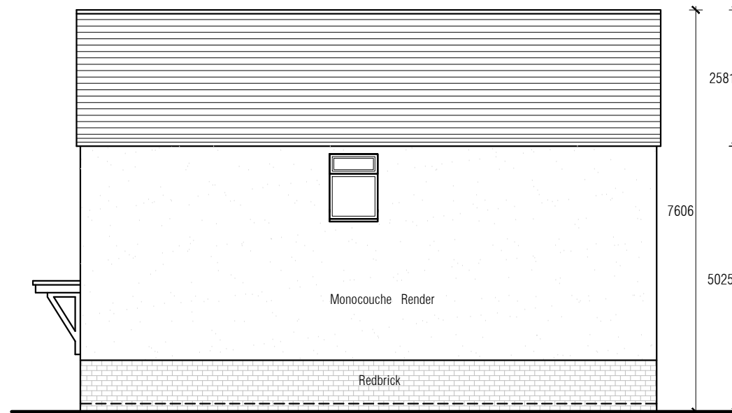
PROPOSED SIDE ELEVATION.RHS PLOT 2
