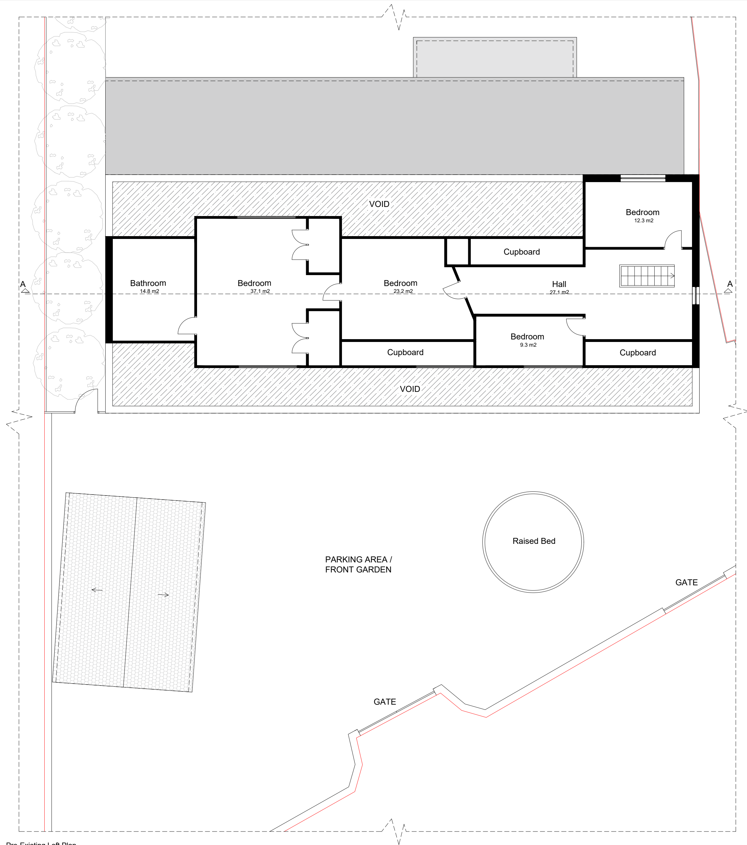
Pre-Existing Loft Plan
