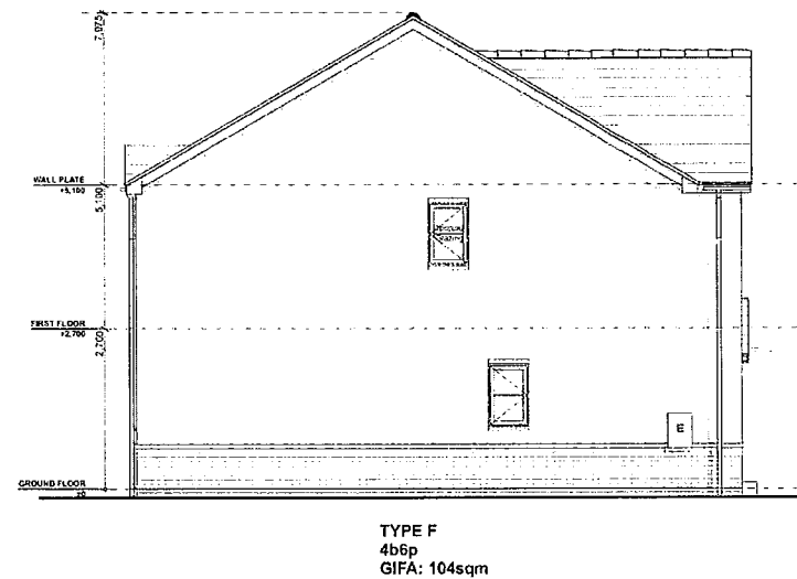
GABLE 2 ELEVATION 1:100
