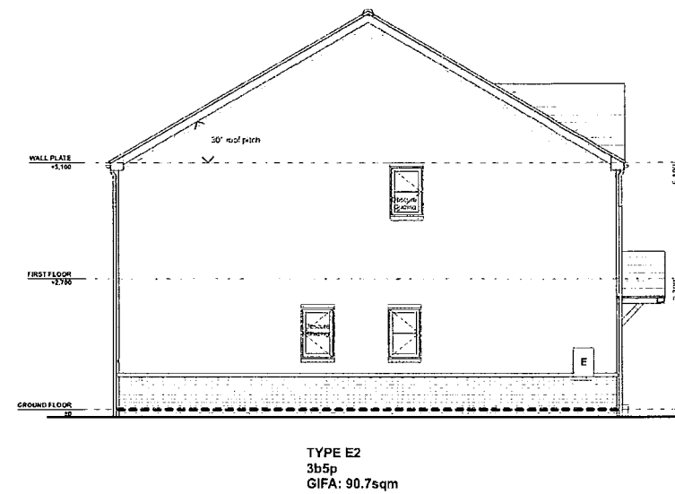
GABLE 1 ELEVATION 1:100
