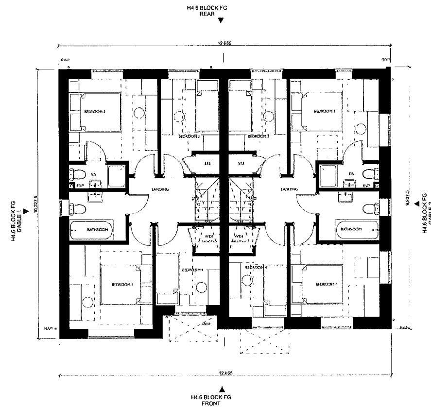
BLOCK FG FIRST FLOOR 1:100
