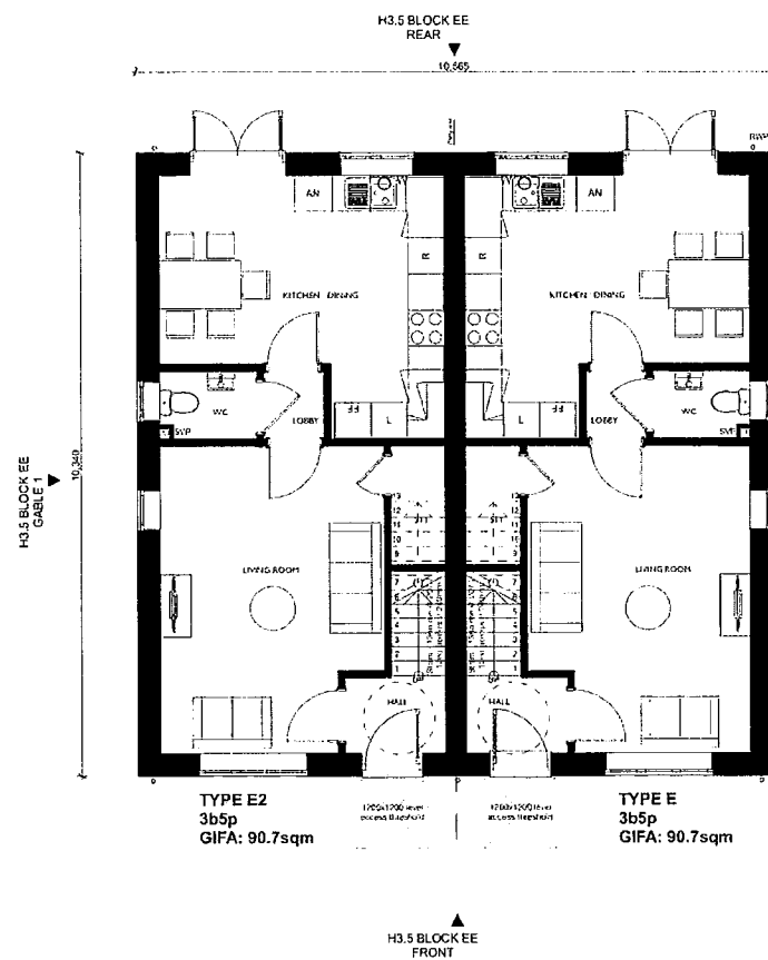
BLOCK E2E GROUND FLOOR 1:100
