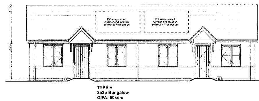
FRONT ELEVATION 1:100
