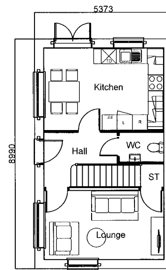
2B4P CT - GIFA: 77sqm GROUND FLOOR
