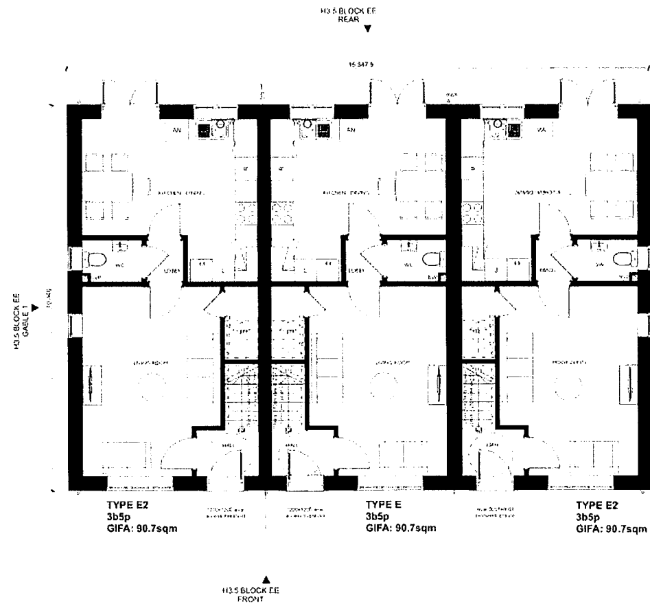
BLOCK E2E GROUND FLOOR 1:100
