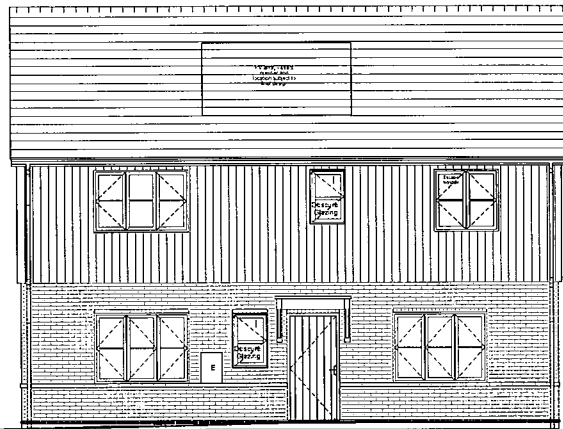
3B5P CT SIDE ELEVATION Plot 19
