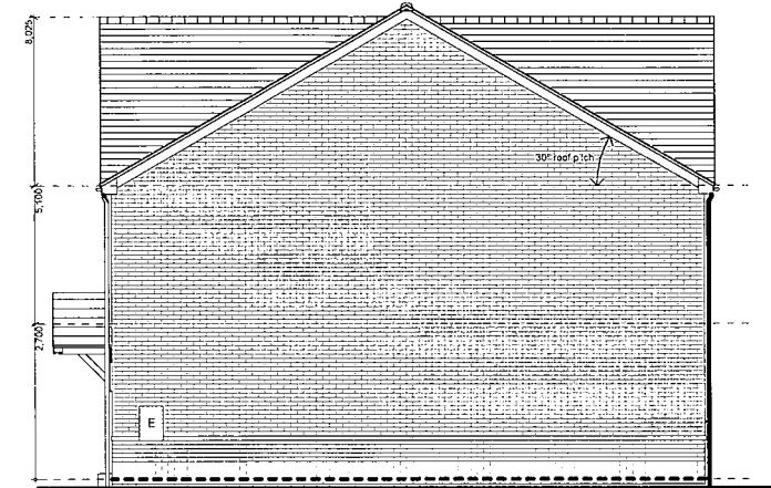
3B5P SIDE ELEVATION Plot 20
