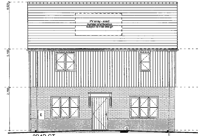
2B4P CT FRONT ELEVATION
