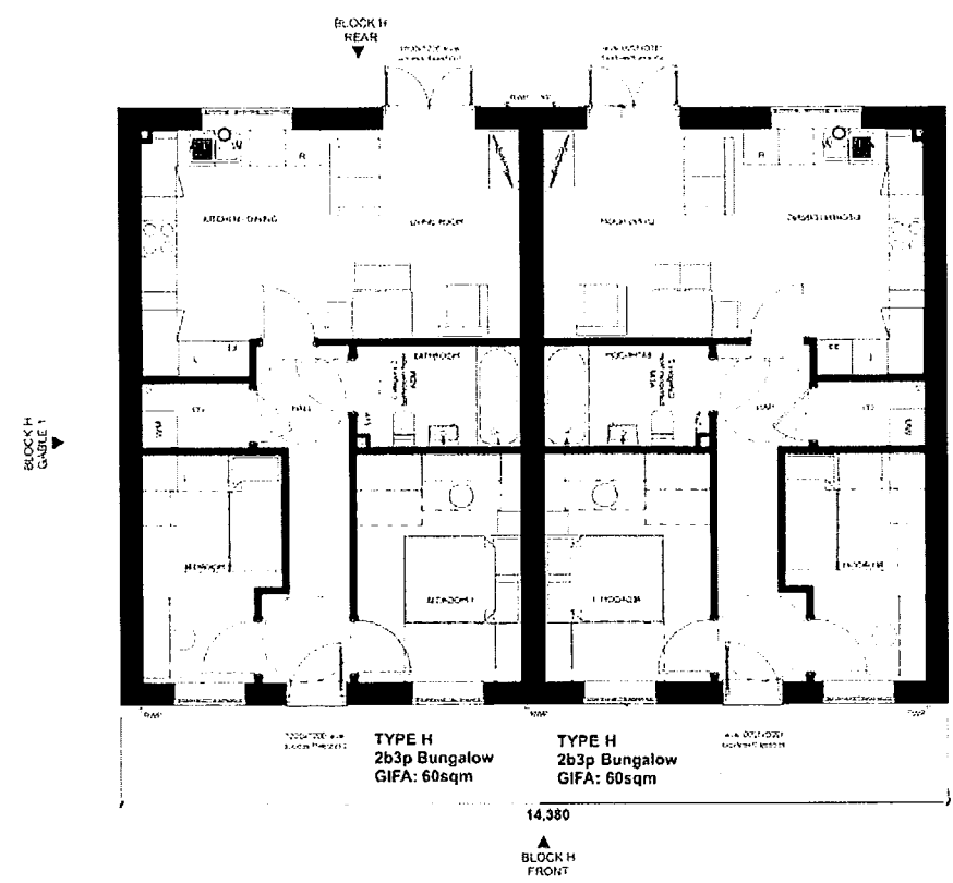
BLOCK H GROUND FLOOR 1:100
