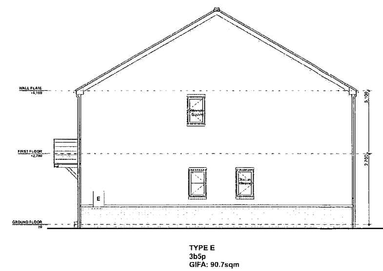
GABLE 2 ELEVATION 1:100
