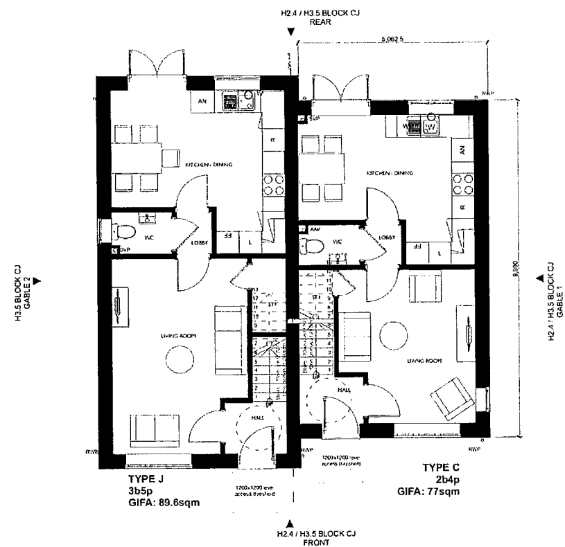
BLOCK CJ GROUND FLOOR 1:100
