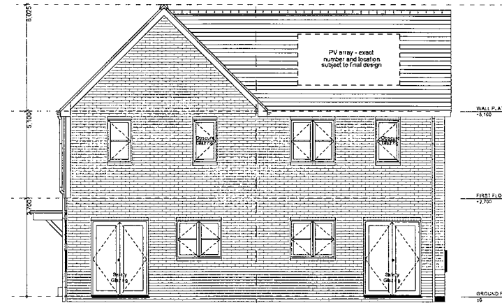
1:100 2B4P CT REAR ELEVATION Plot 28
