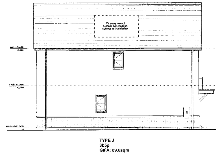
Gable 2 Elevation 1:100
