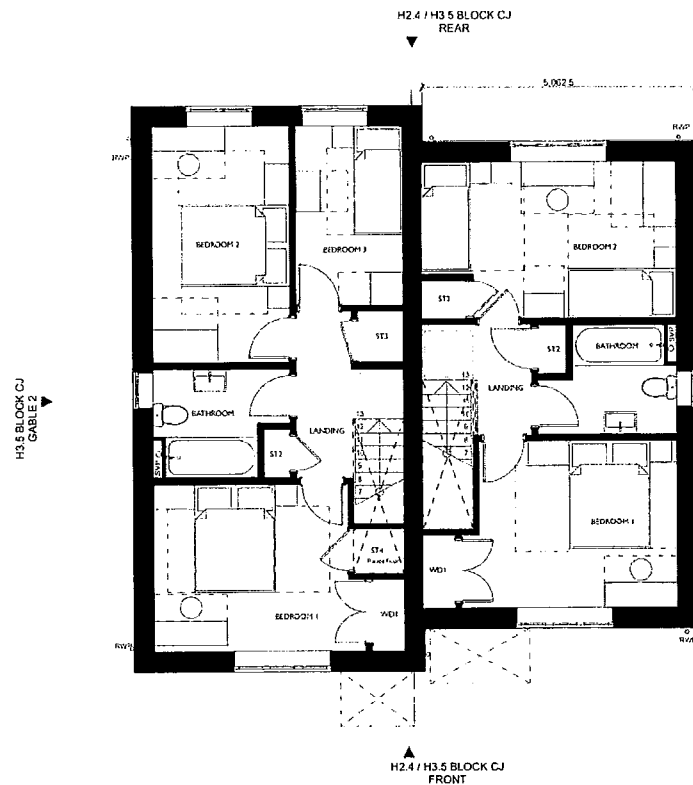
BLOCK CJ FIRST FLOOR 1:100
