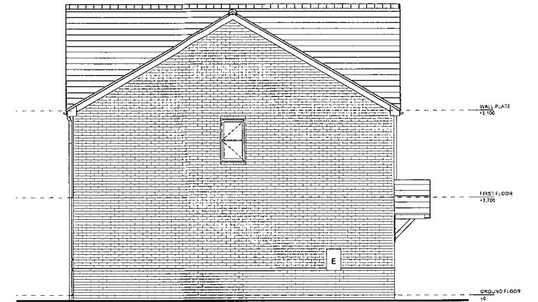
1:100 2B4P GABLE 2 ELEVATION Plot 27
