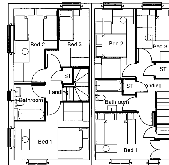
3B5P CT FIRST FLOOR
