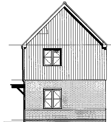
2B4P CT SIDE ELEVATION Plot 11
