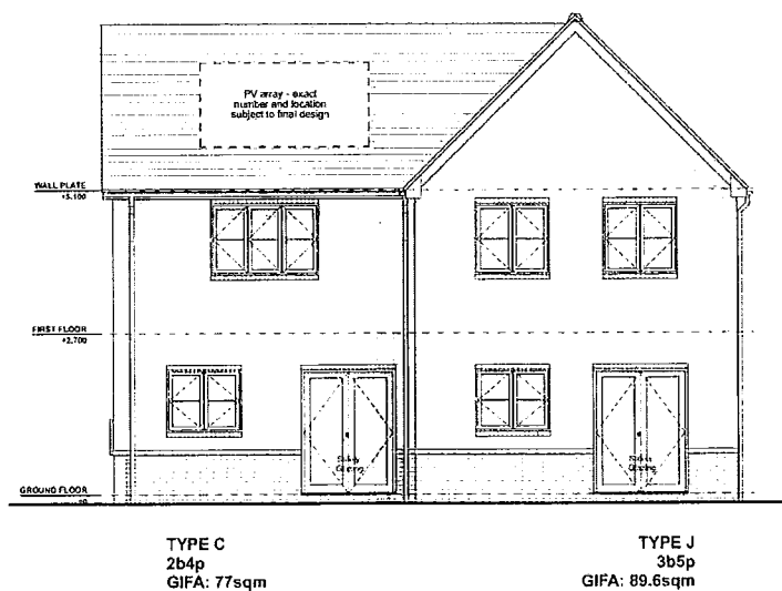
Rear Elevation 1:100
