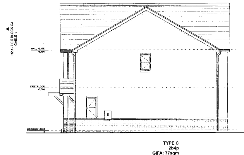
Gable 1 Elevation 1:100
