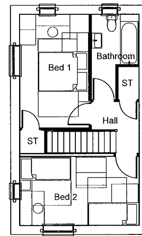
2B4P CT FIRST FLOOR
