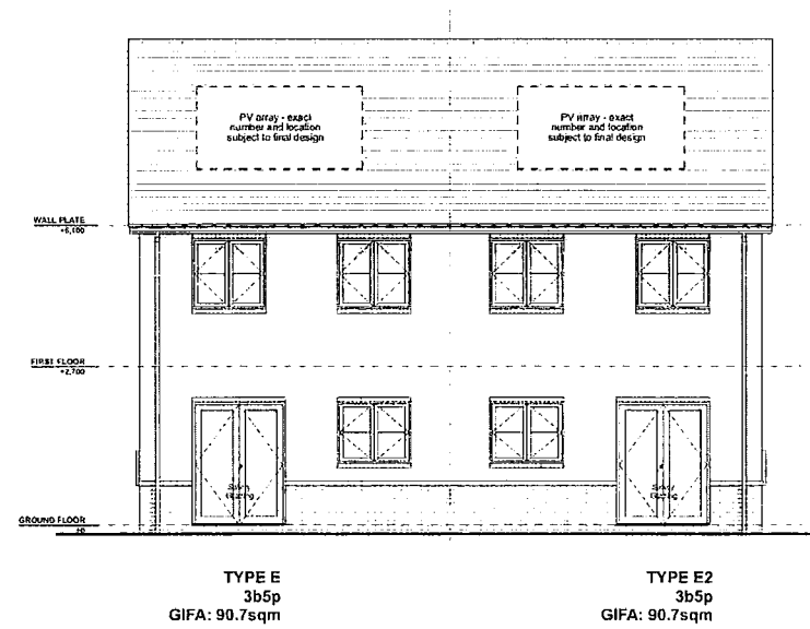
REAR ELEVATION 1:100
