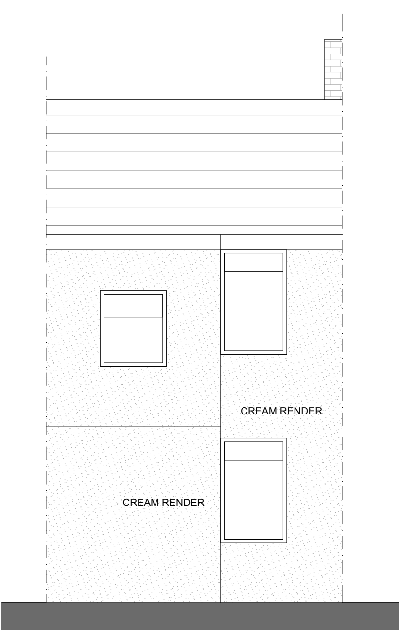
PROPOSED BACK ELEVATION
