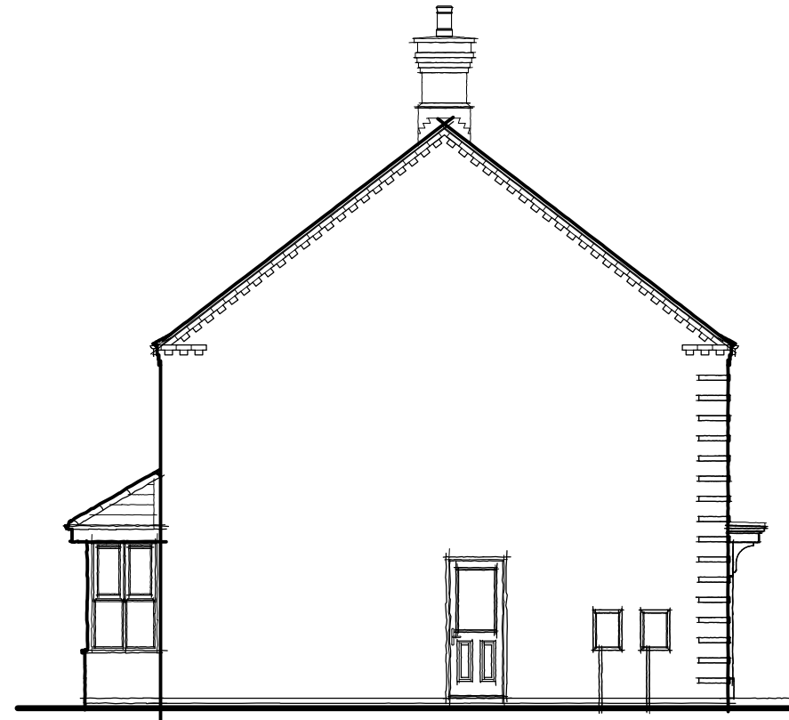
Side Elevation
