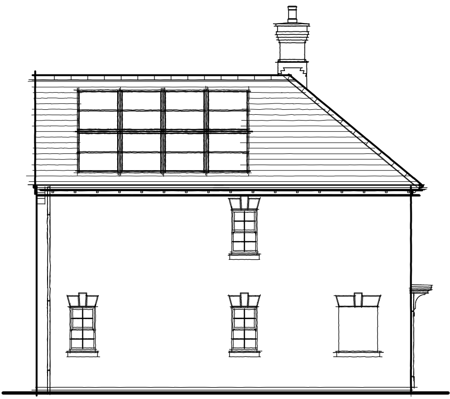
Side Elevation
