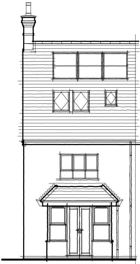
Rear Elevation
