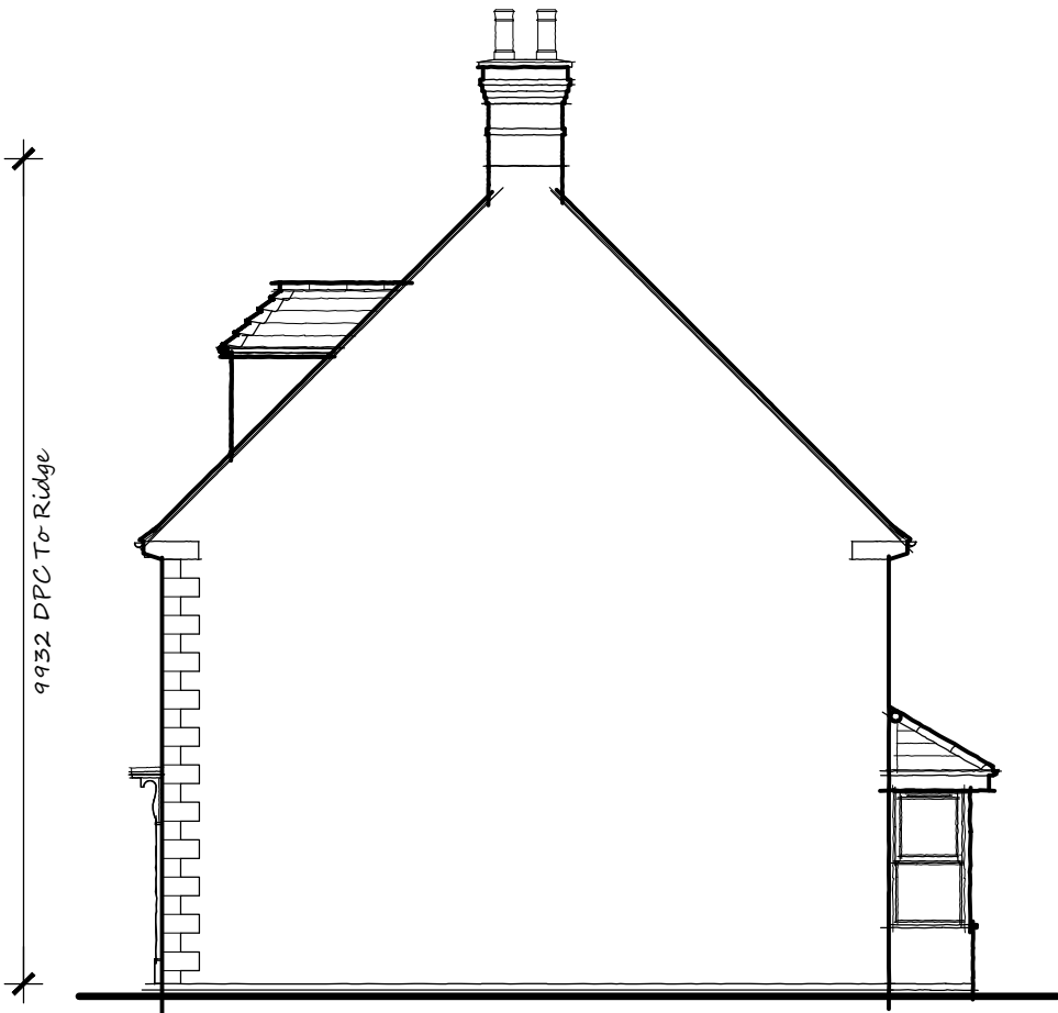
Side Elevation
