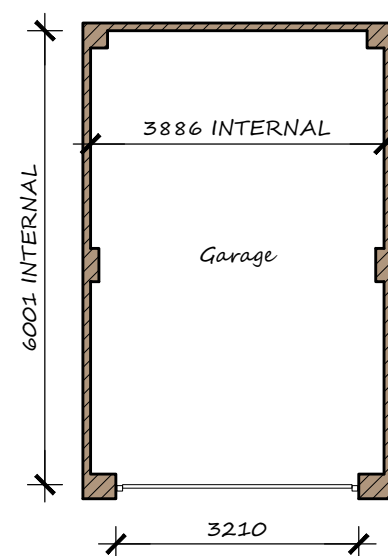
Floor Plan
