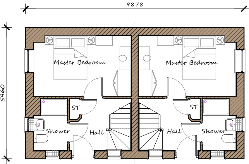
DH16GEA-5 Ground Floor Plans
