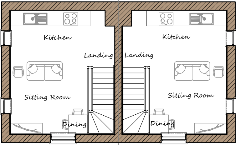
DH16GEA-5 First Floor Plans
